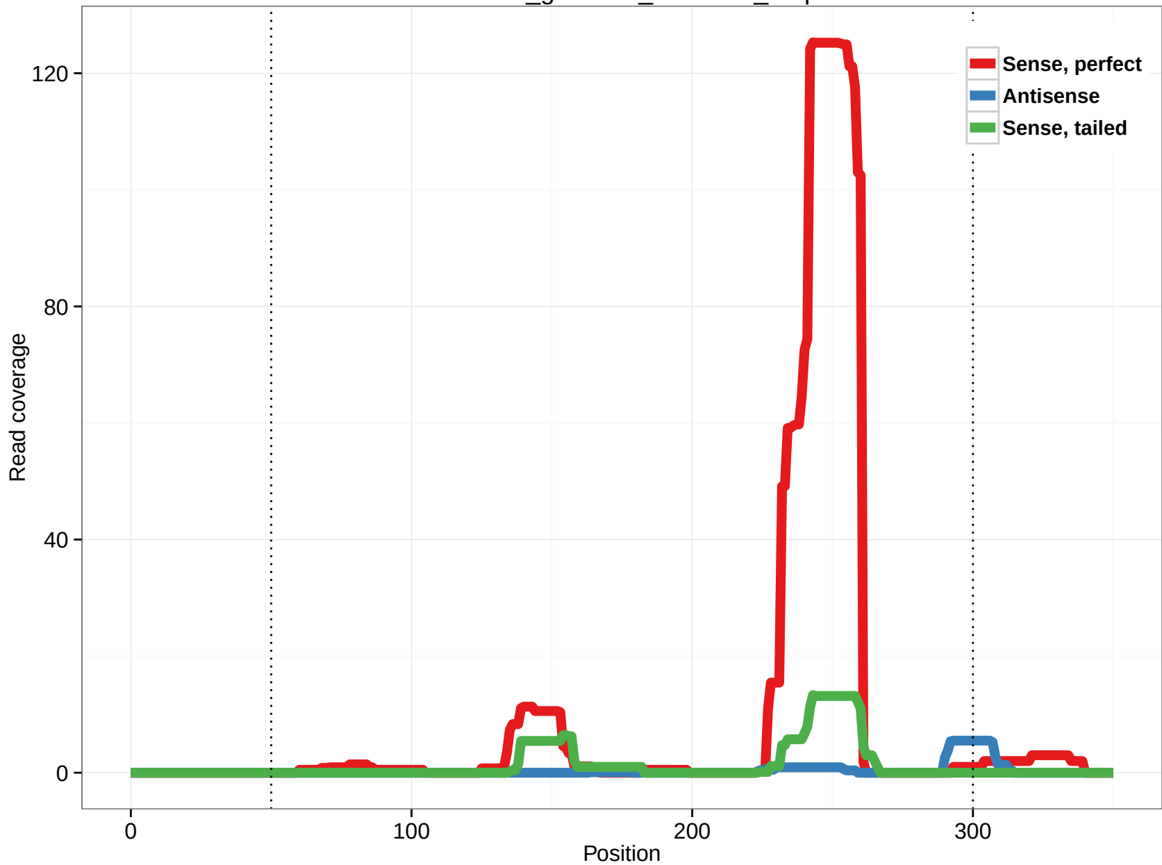
rheMac3_genscan_chr7.125_1.3p
