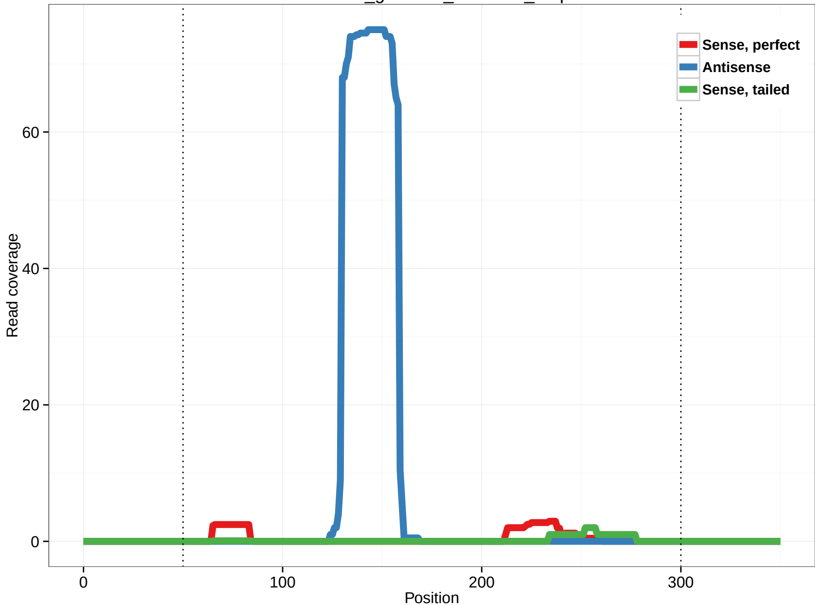
rheMac3_genscan_chr7.125_0.3p
