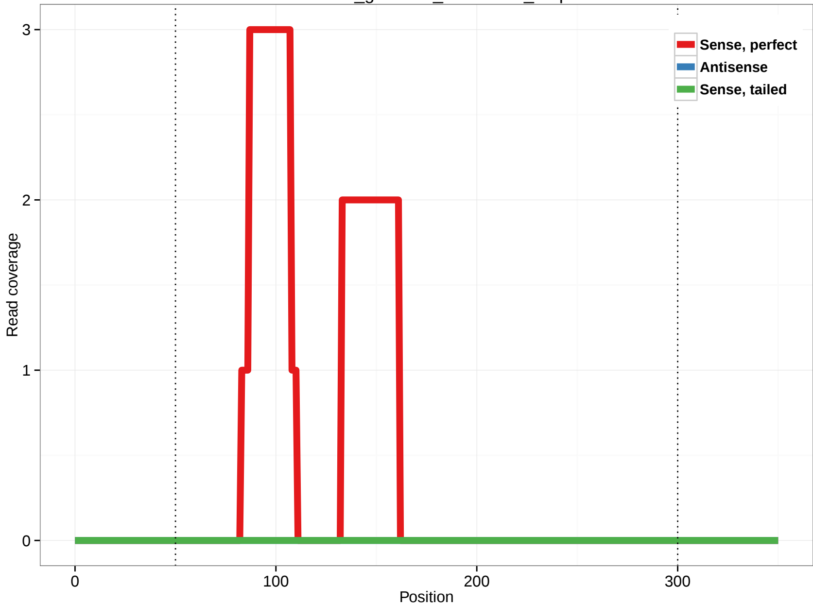
rheMac3_genscan_chr7.1254_1.3p
