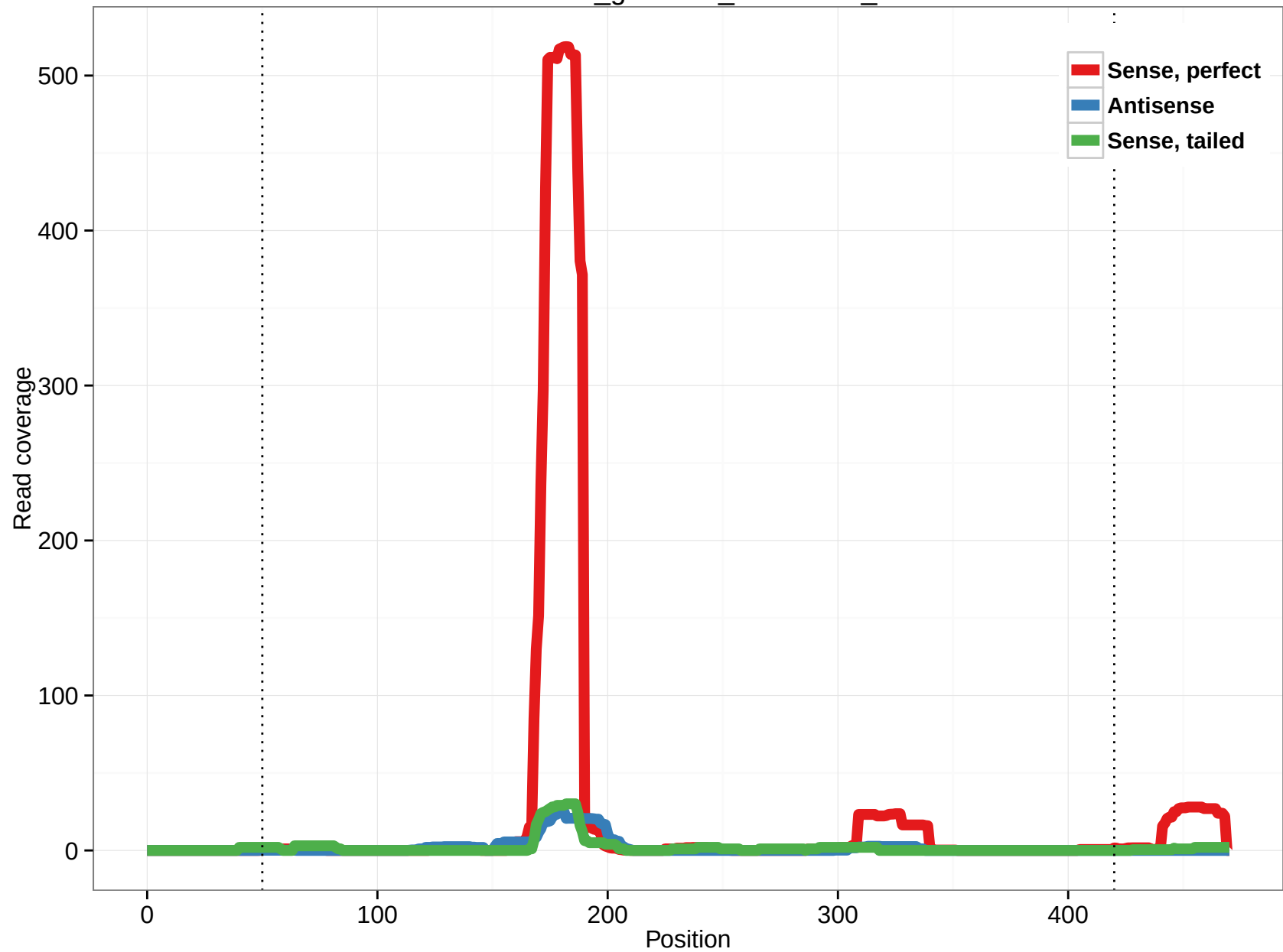
rheMac3_genscan_chr7.1245_9
