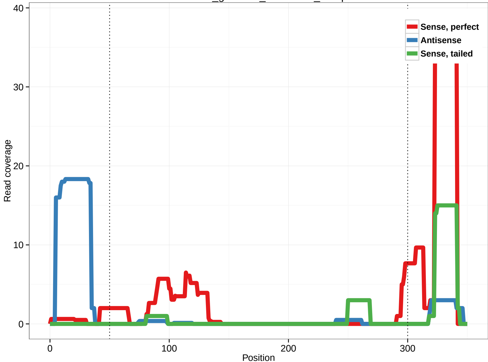
rheMac3_genscan_chr7.1245_11.3p
