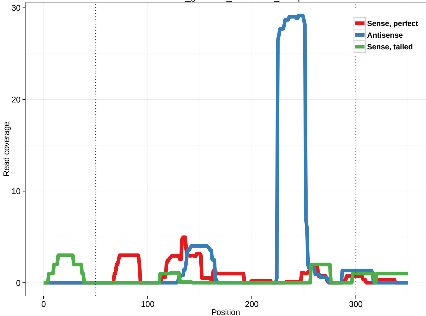
rheMac3_genscan_chr7.1245_10.5p
