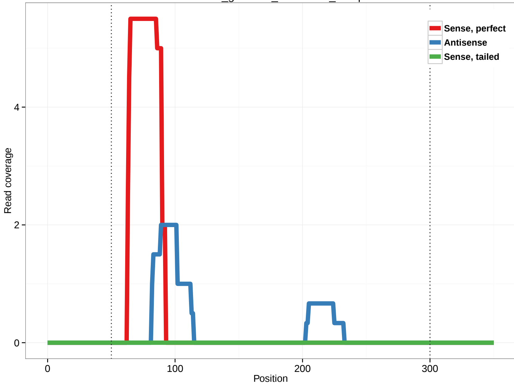
rheMac3_genscan_chr7.1239_20.5p
