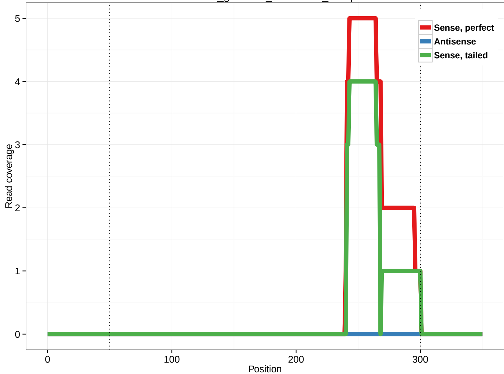
rheMac3_genscan_chr7.1168_28.3p
