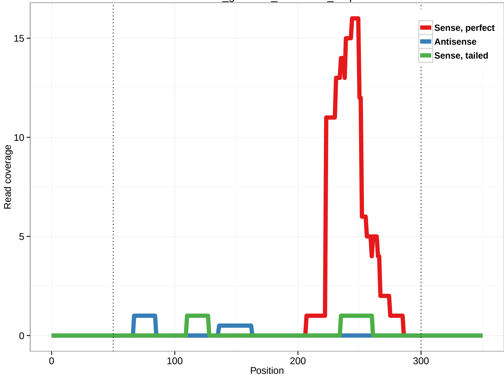
rheMac3_genscan_chr7.1164_1.5p
