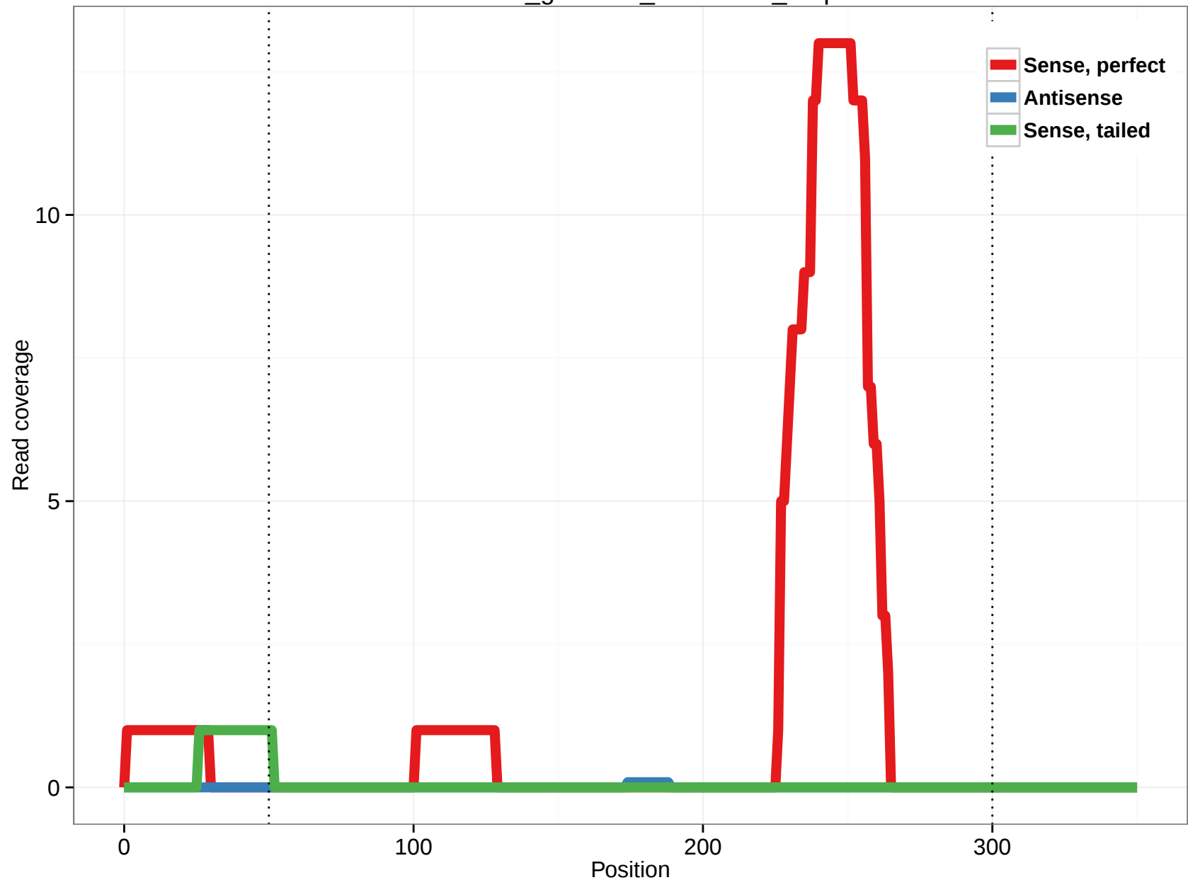
rheMac3_genscan_chr7.1148_6.5p
