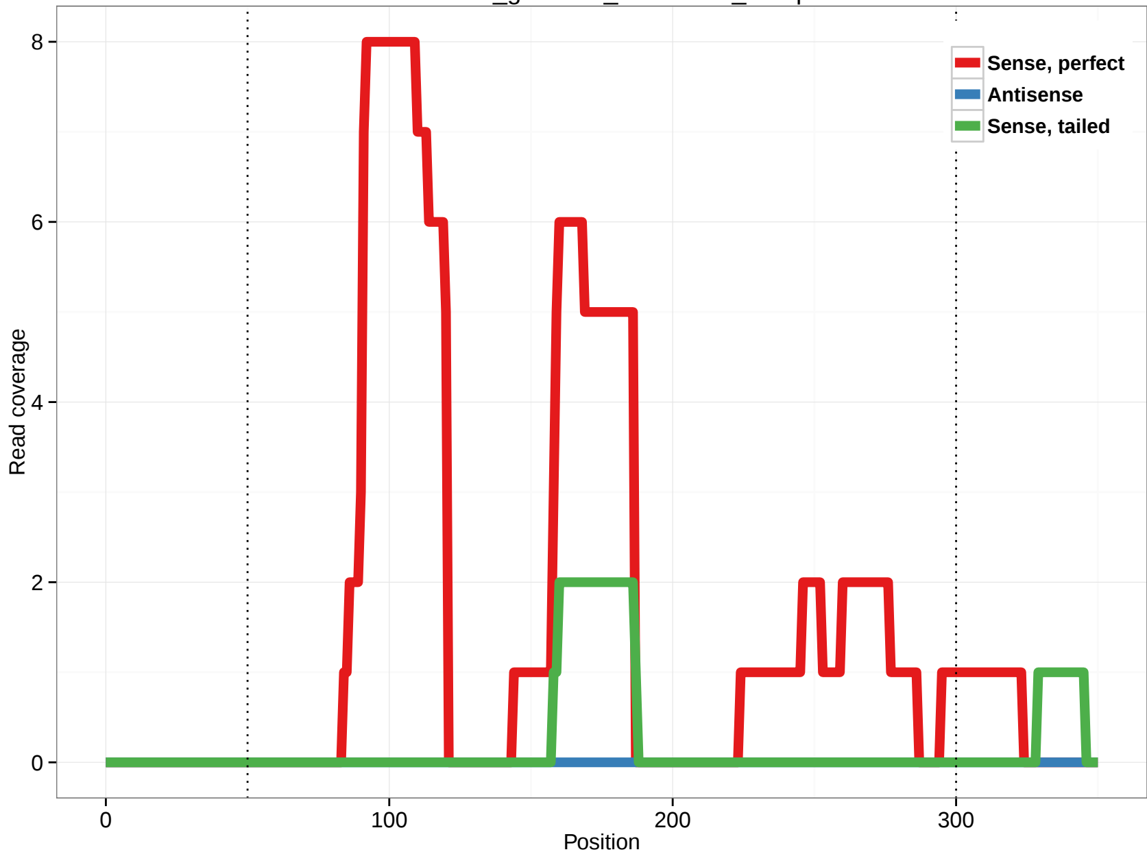
rheMac3_genscan_chr7.1147_10.5p
