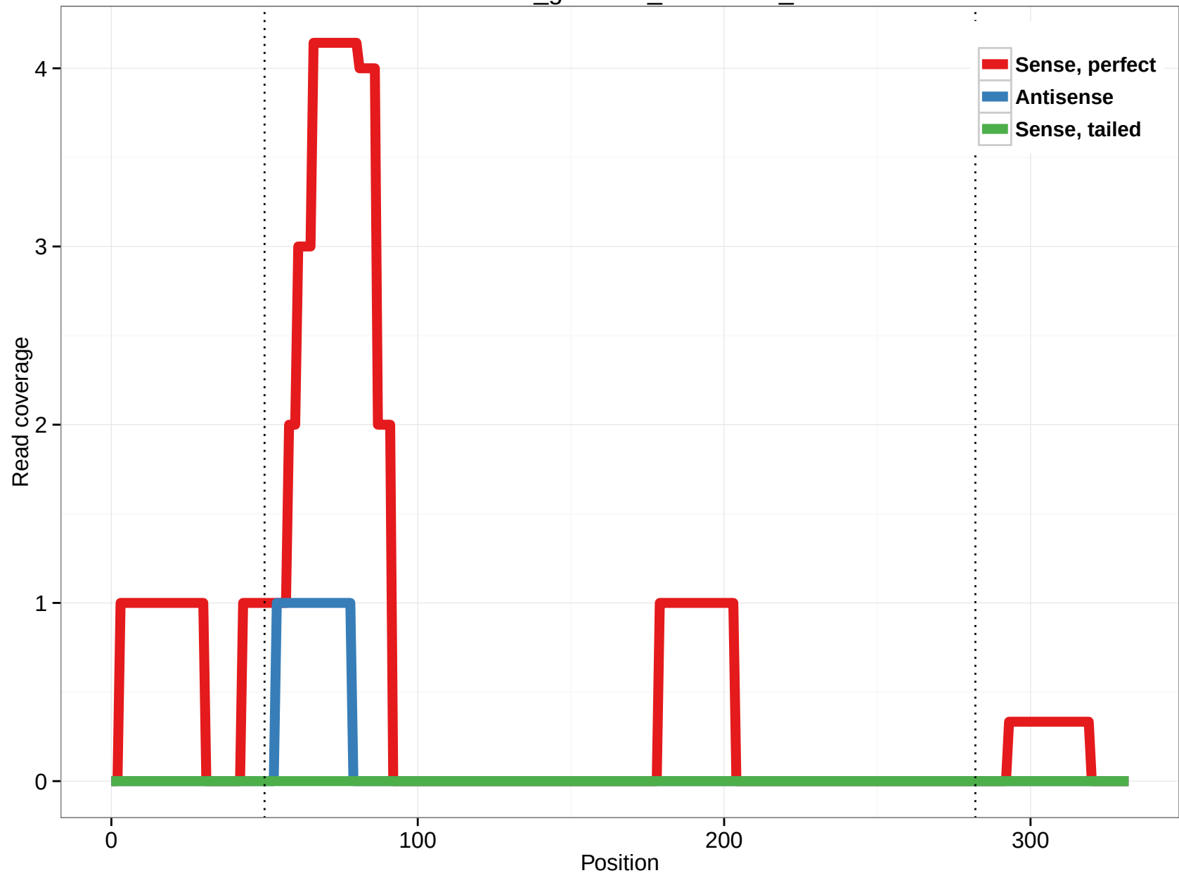
rheMac3_genscan_chr7.1133_4
