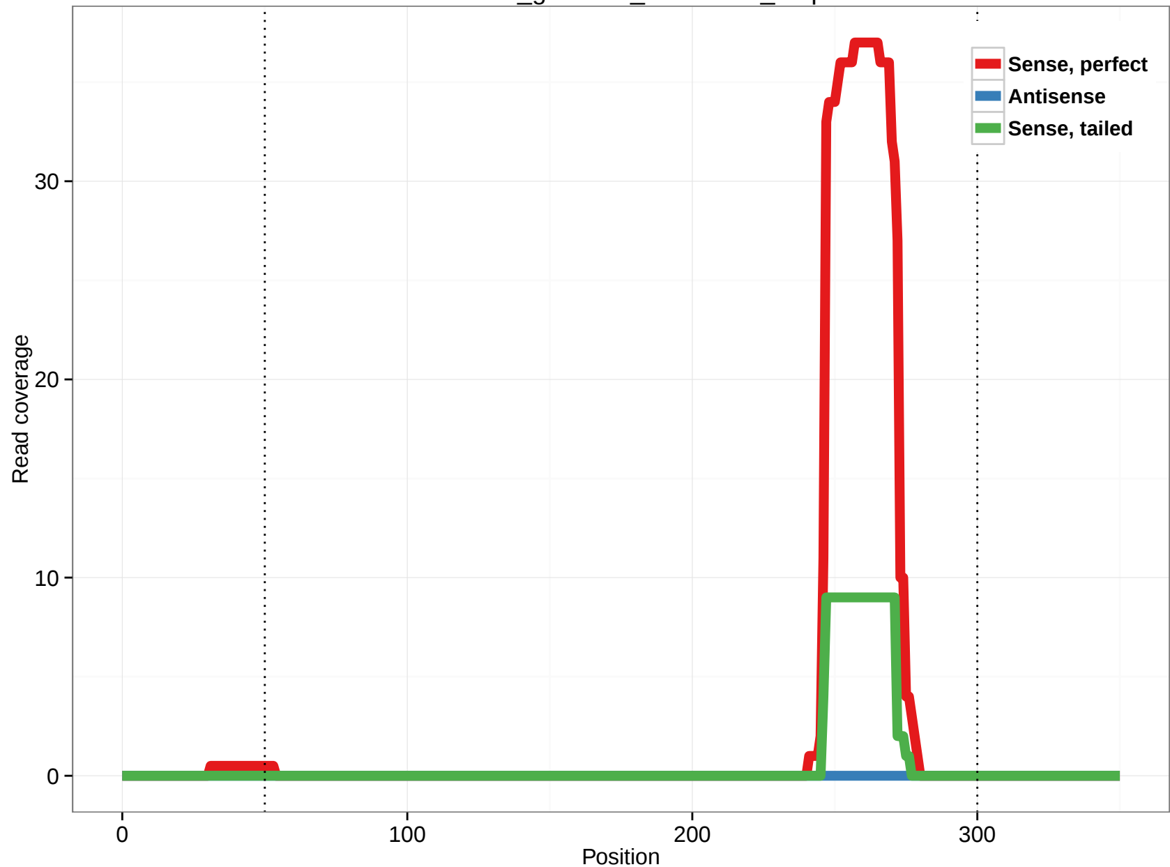
rheMac3_genscan_chr7.1133_0.3p
