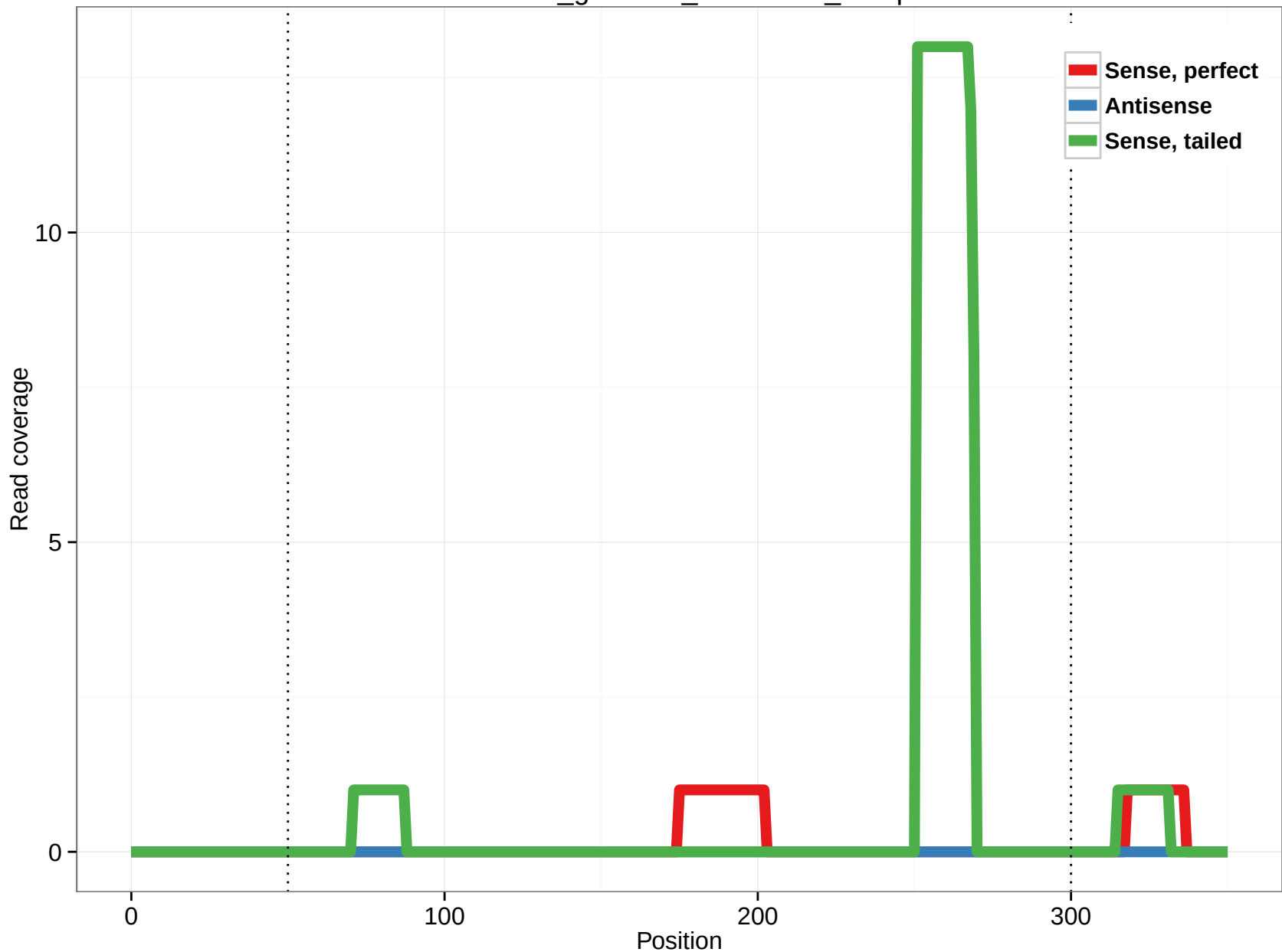
rheMac3_genscan_chr7.1122_20.5p
