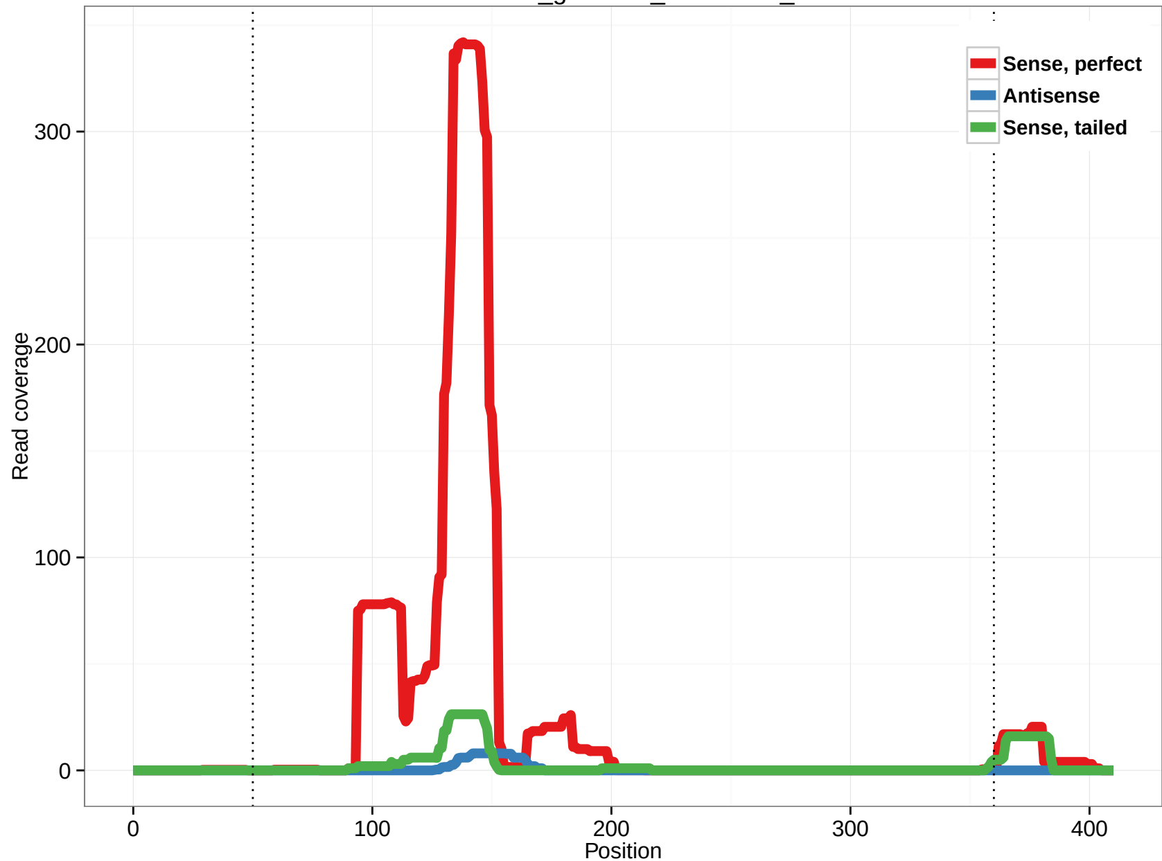
rheMac3_genscan_chr7.1104_3
