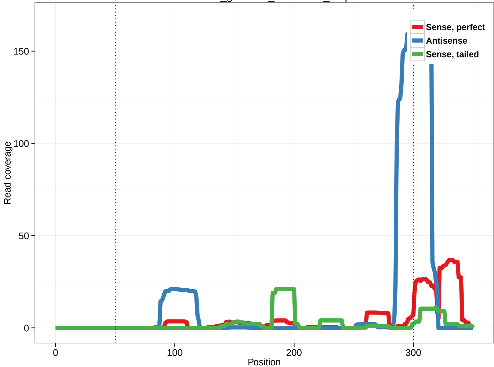
rheMac3_genscan_chr7.1098_4.5p
