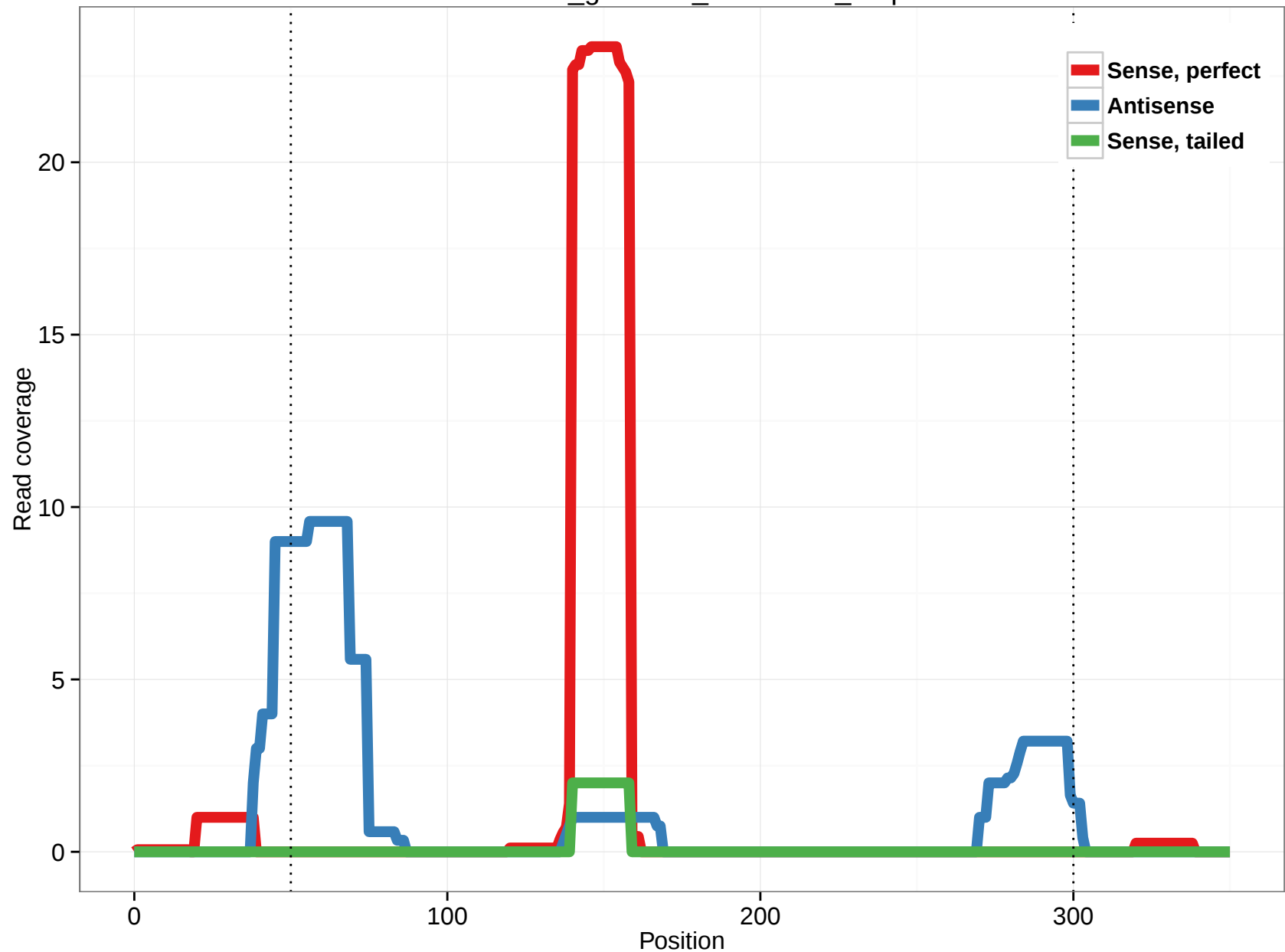
rheMac3_genscan_chr7.1098_2.3p
