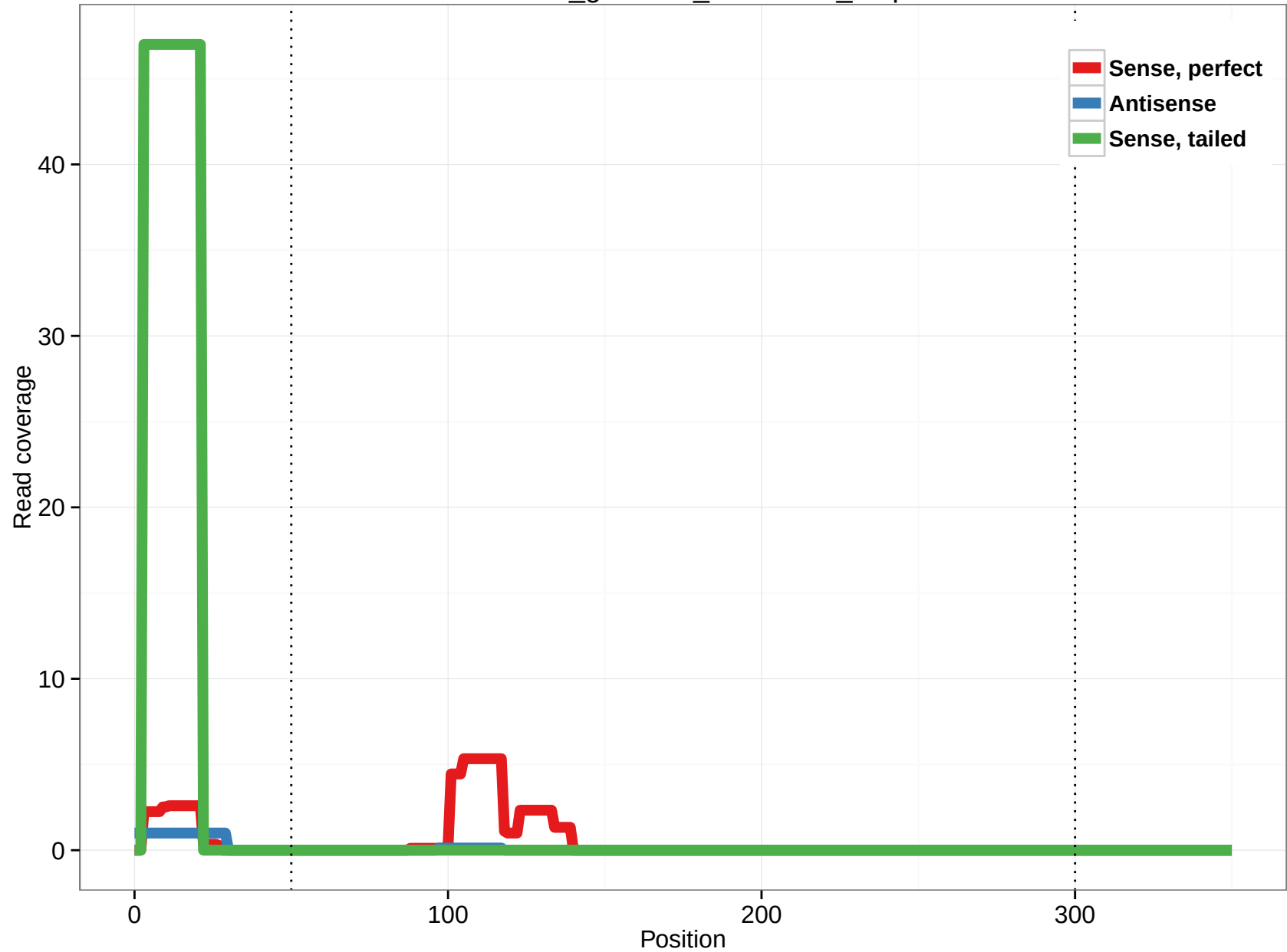
rheMac3_genscan_chr7.1098_1.5p
