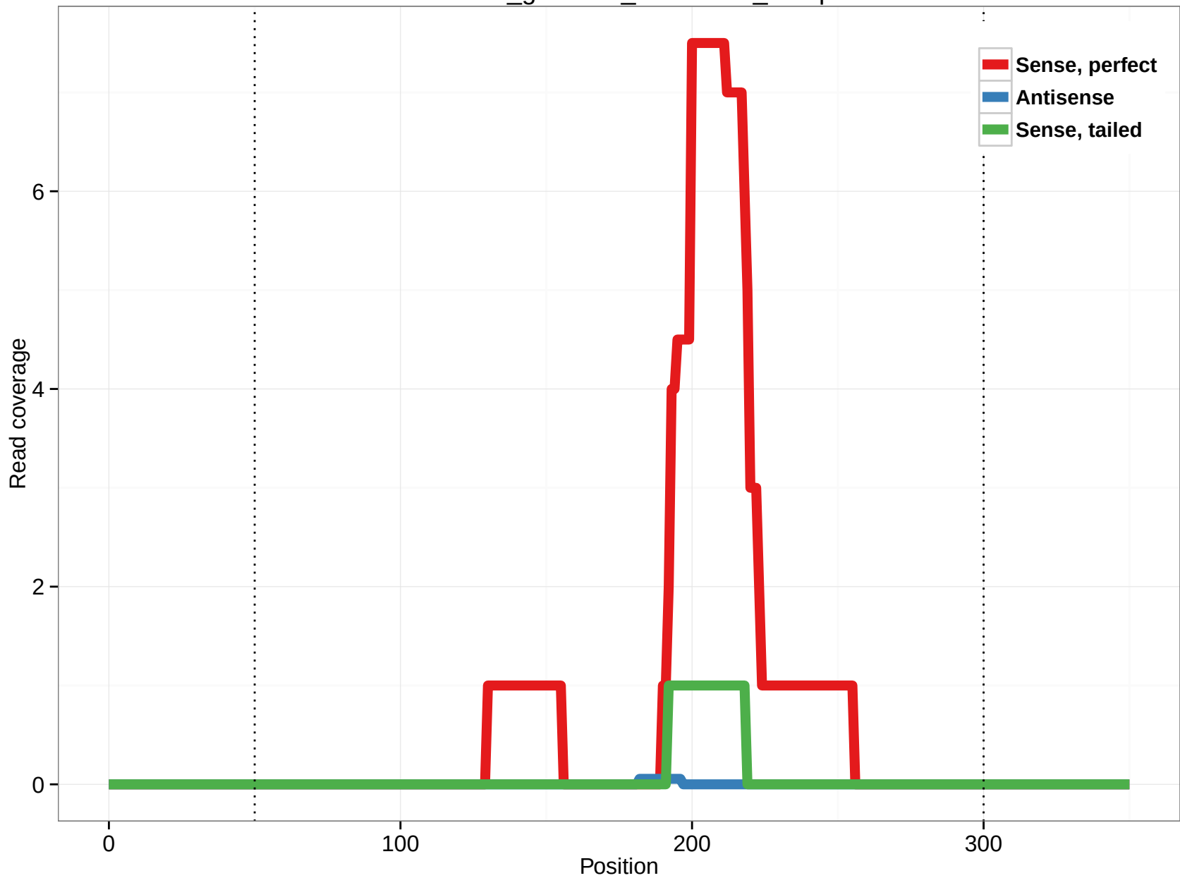
rheMac3_genscan_chr7.1096_17.3p
