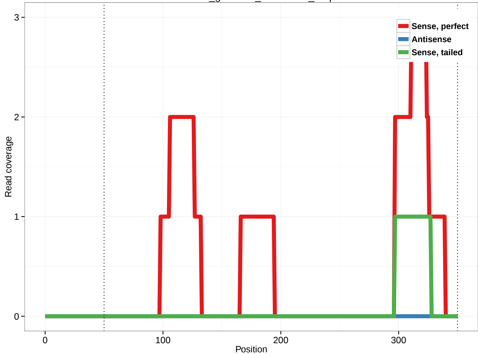
rheMac3_genscan_chr7.1092_5.5p
