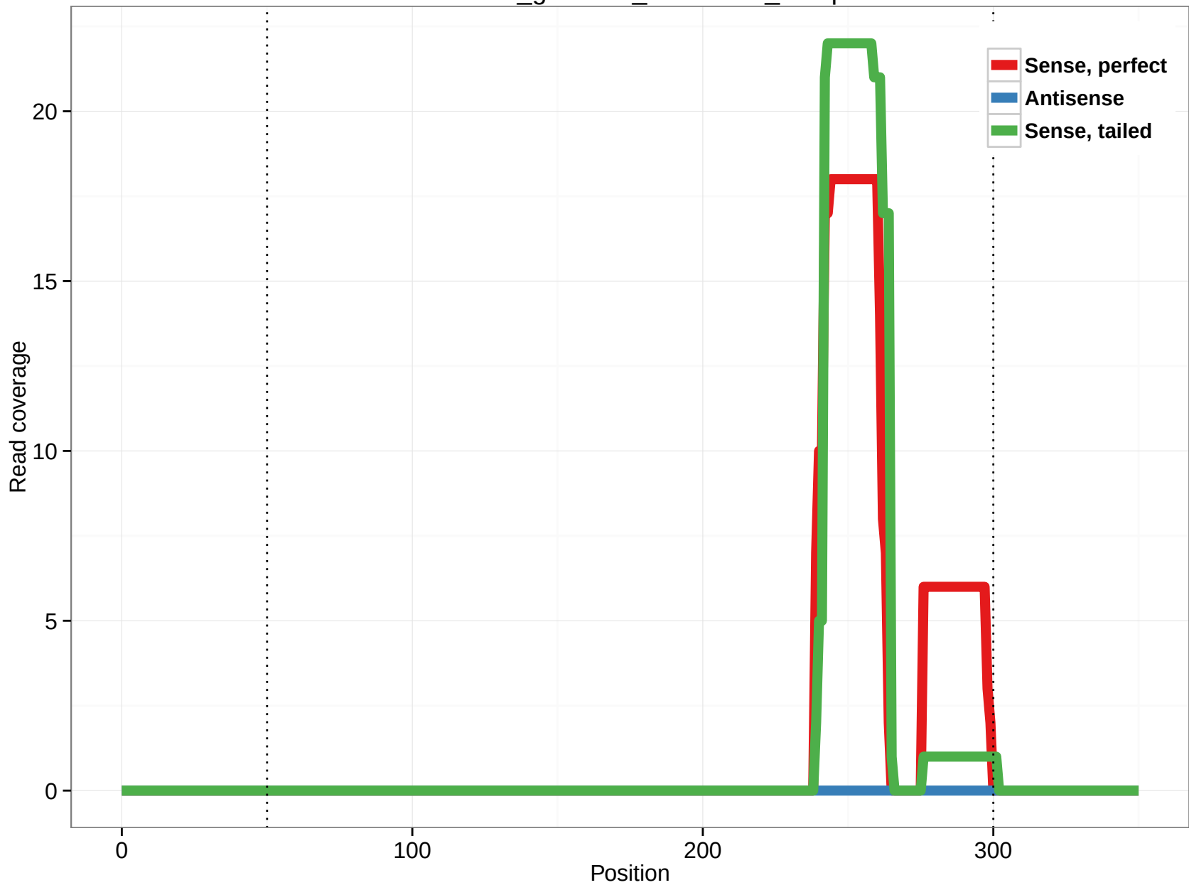
rheMac3_genscan_chr7.1091_12.3p
