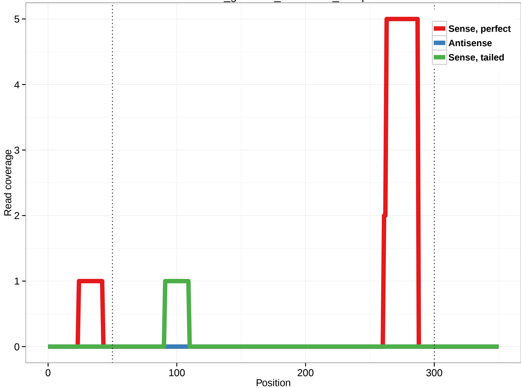
rheMac3_genscan_chr7.1072_15.5p
