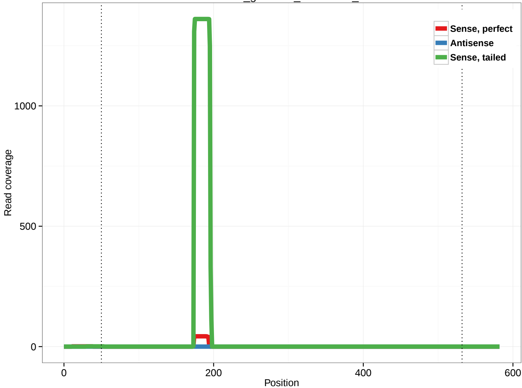
rheMac3_genscan_chr7.1043_6
