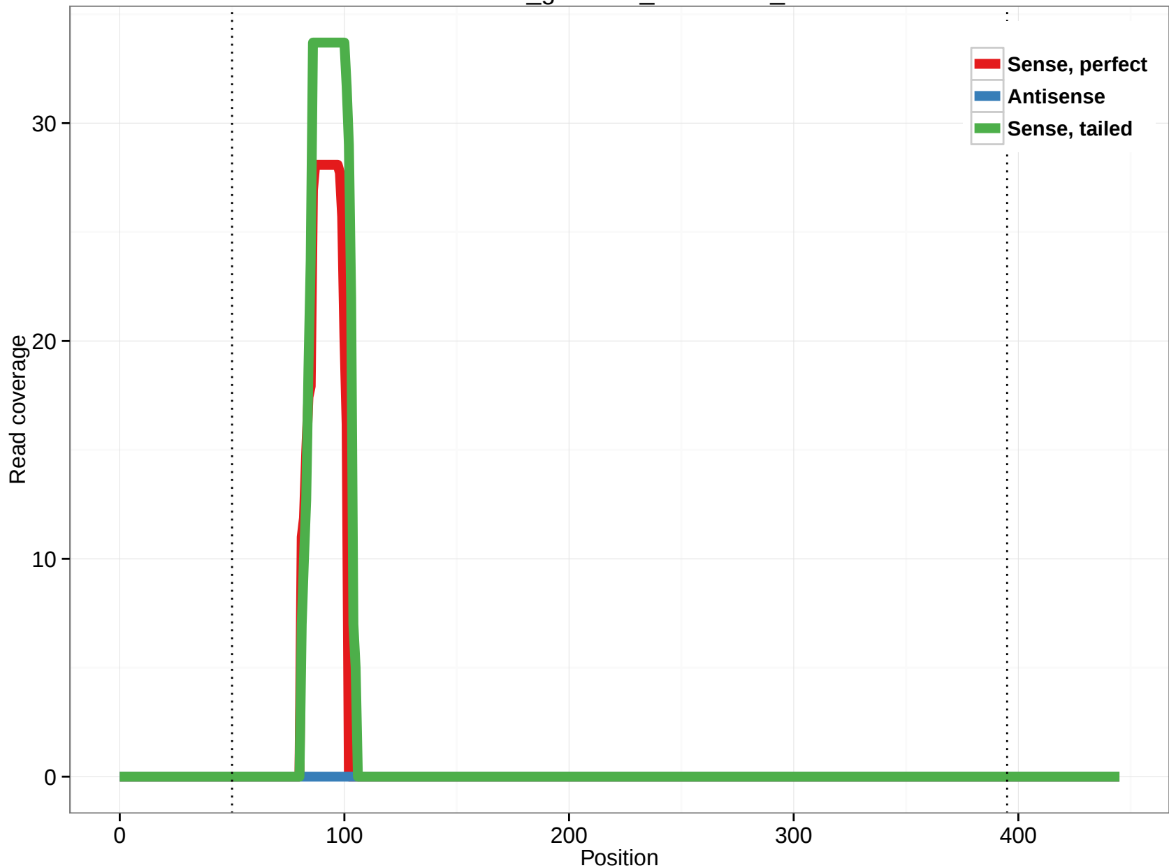
rheMac3_genscan_chr7.1041_18
