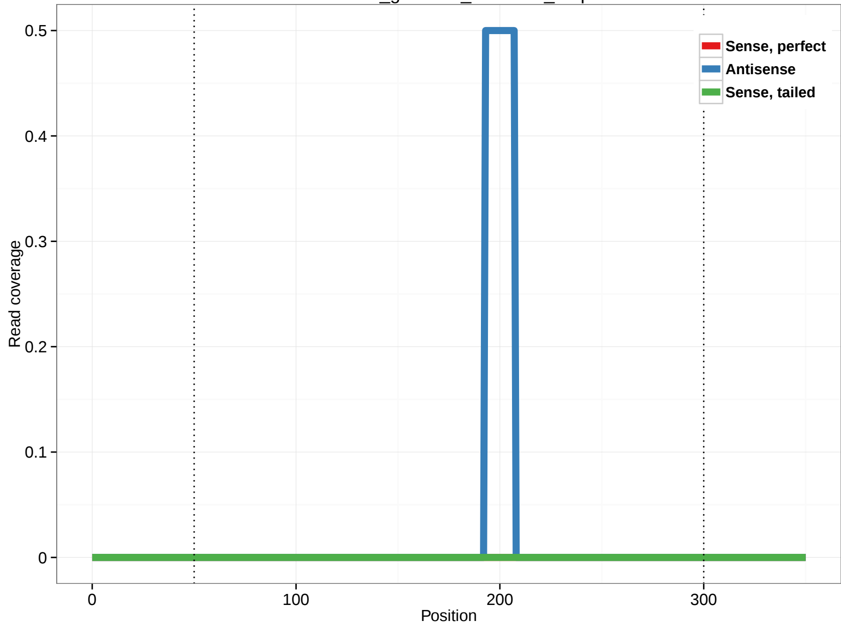
rheMac3_genscan_chr6.995_4.5p
