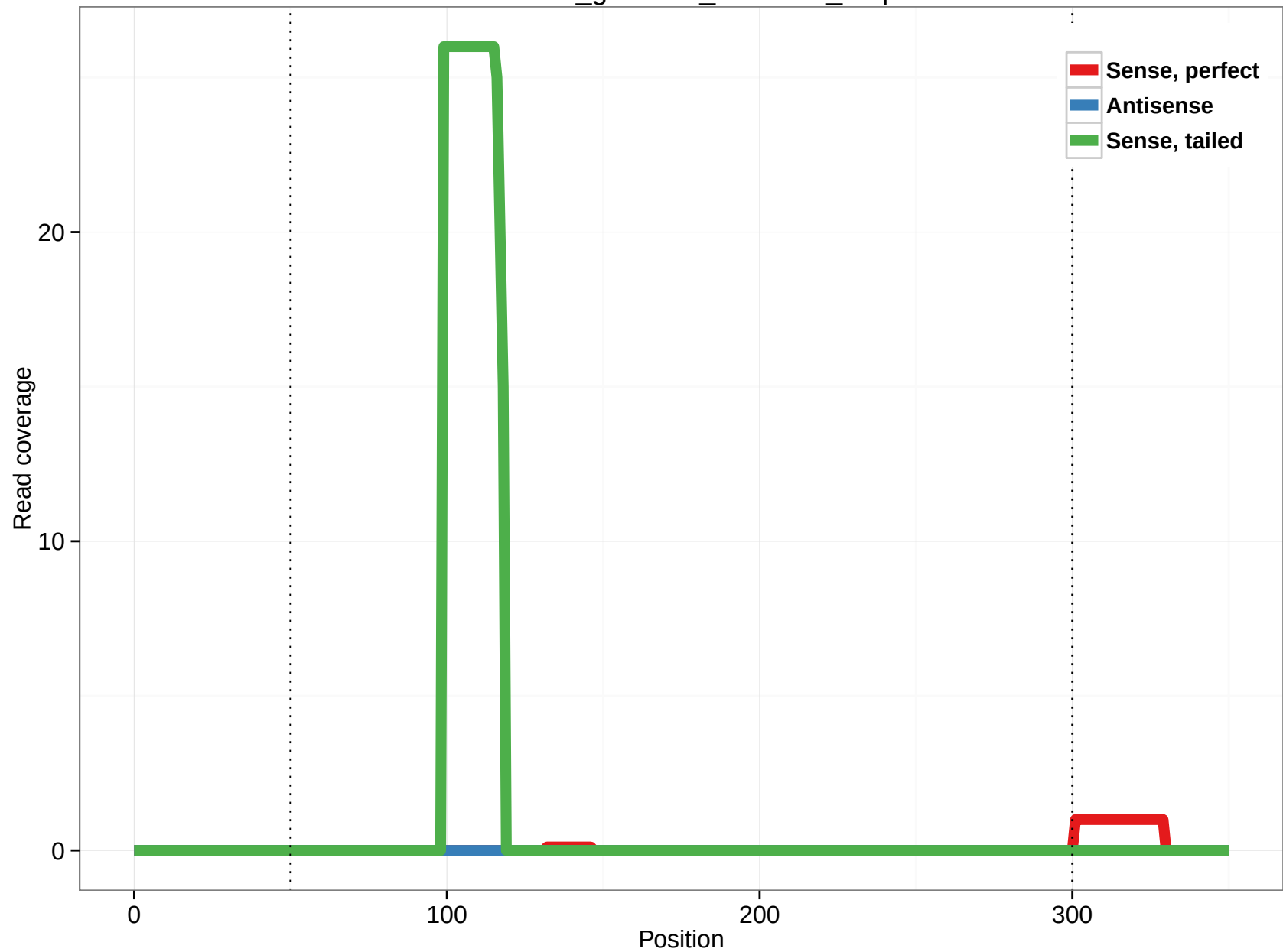
rheMac3_genscan_chr6.923_2.3p
