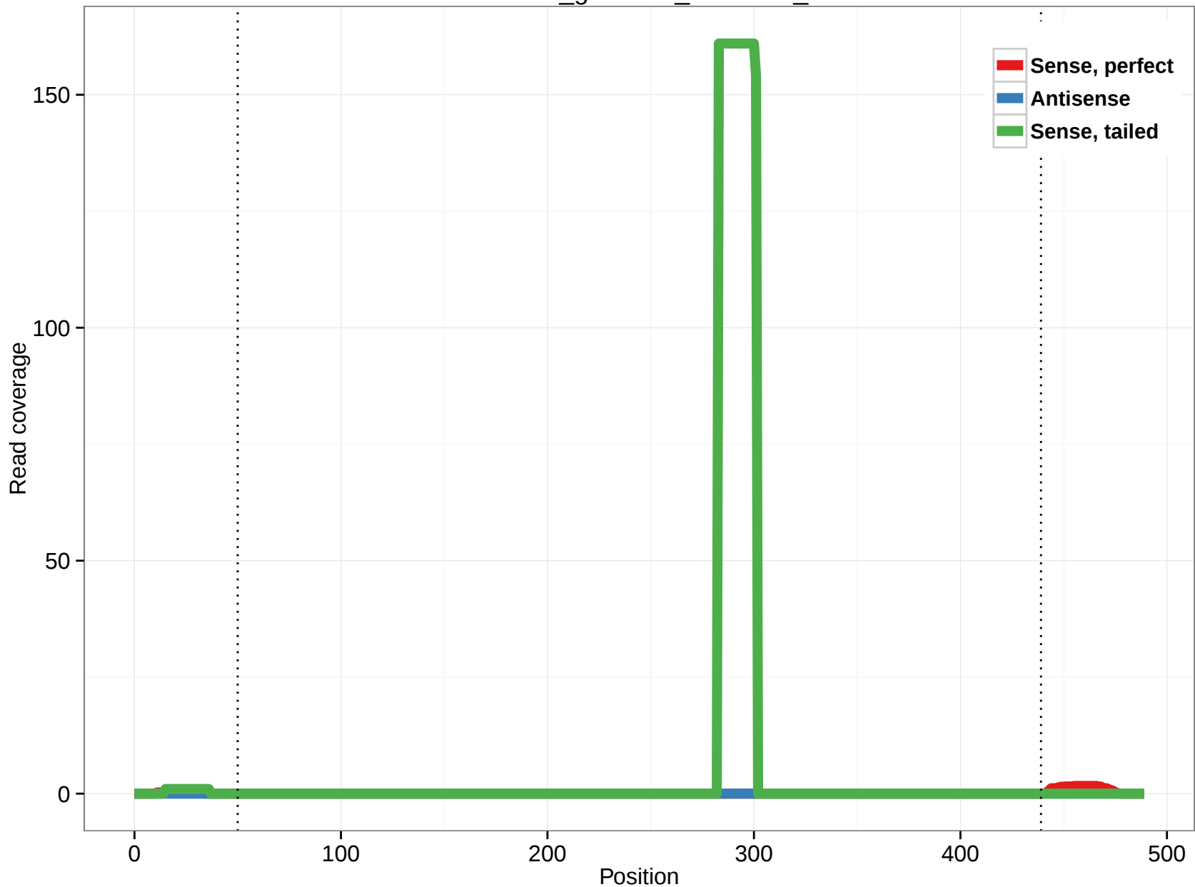
rheMac3_genscan_chr6.843_2
