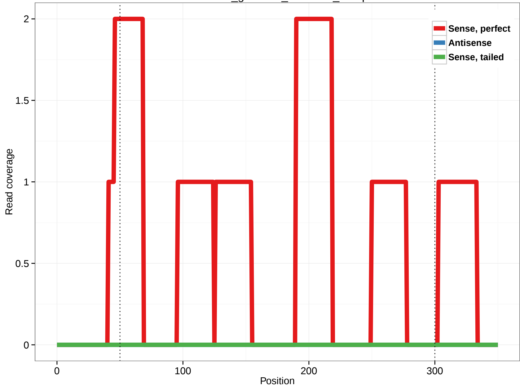
rheMac3_genscan_chr6.808_13.5p
