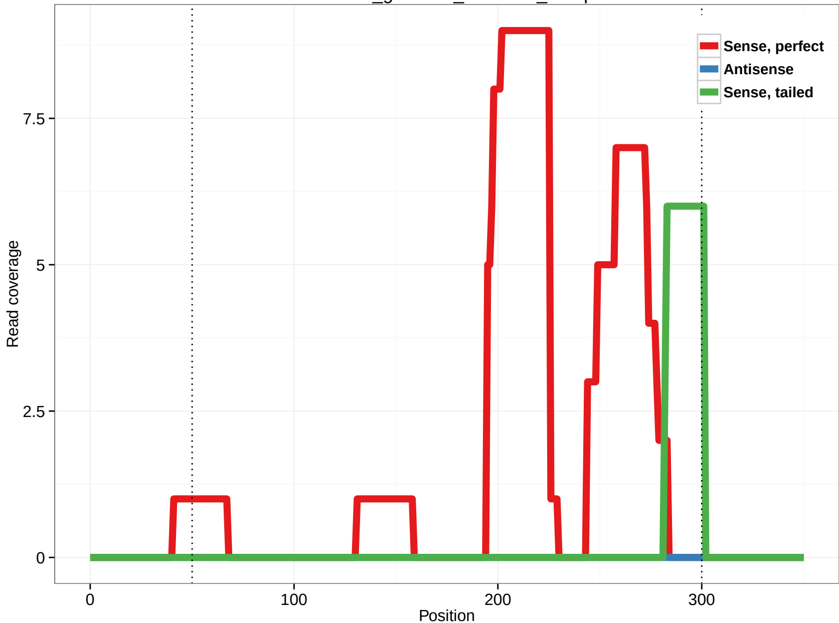
rheMac3_genscan_chr6.808_13.3p
