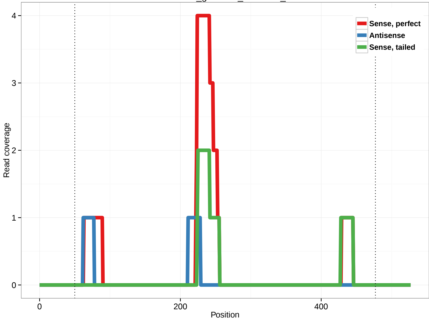
rheMac3_genscan_chr6.794_0
