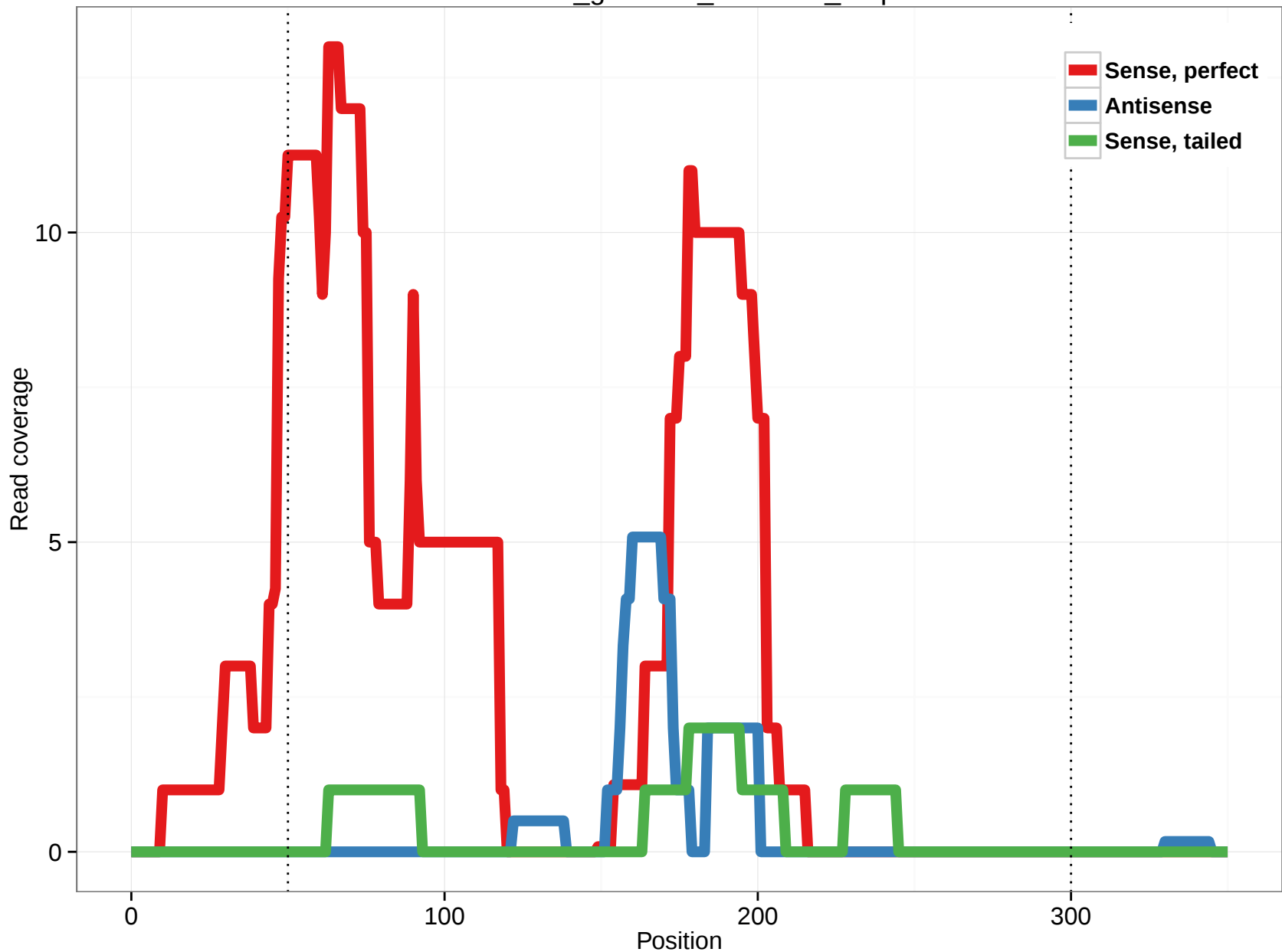
rheMac3_genscan_chr6.706_0.5p
