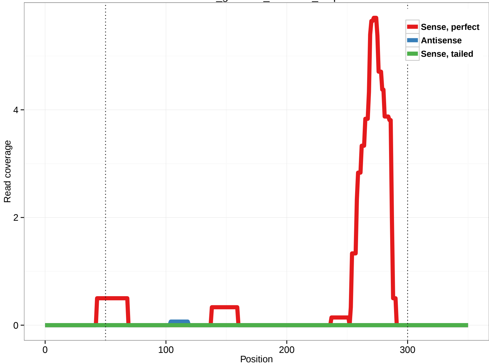
rheMac3_genscan_chr6.698_0.5p
