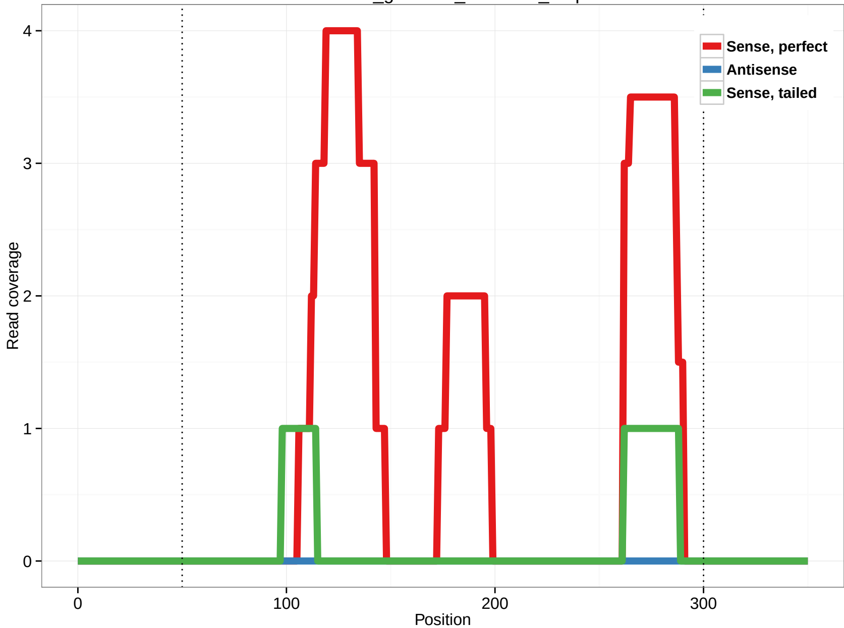
rheMac3_genscan_chr6.659_1.5p
