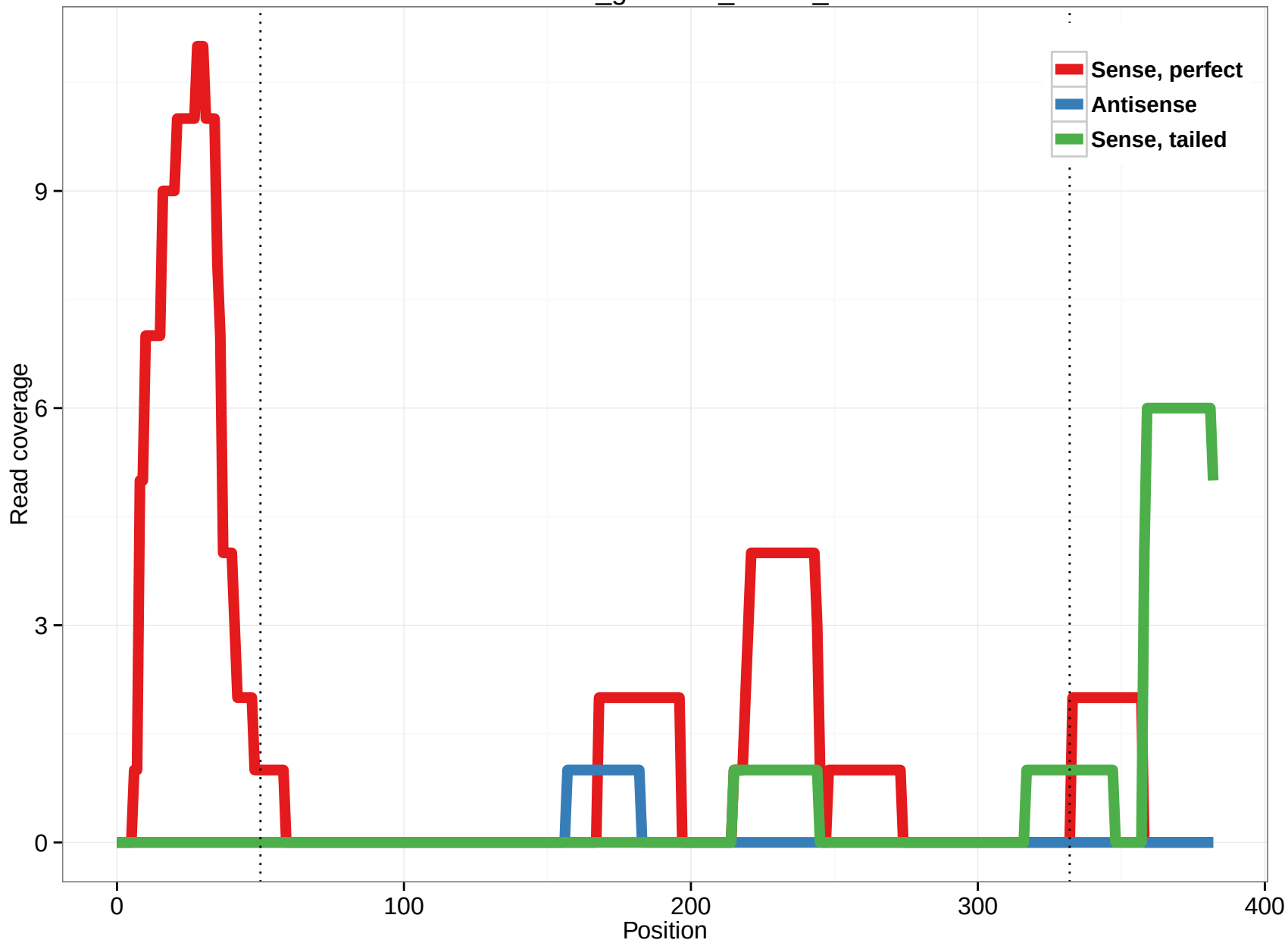
rheMac3_genscan_chr6.5_5
