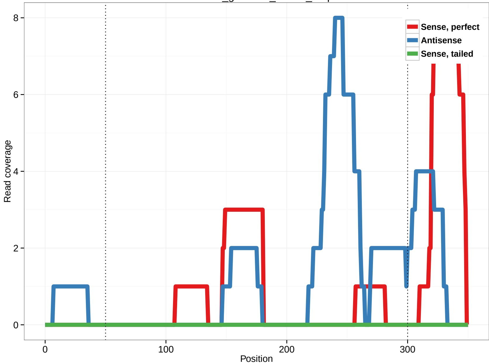
rheMac3_genscan_chr6.5_4.3p
