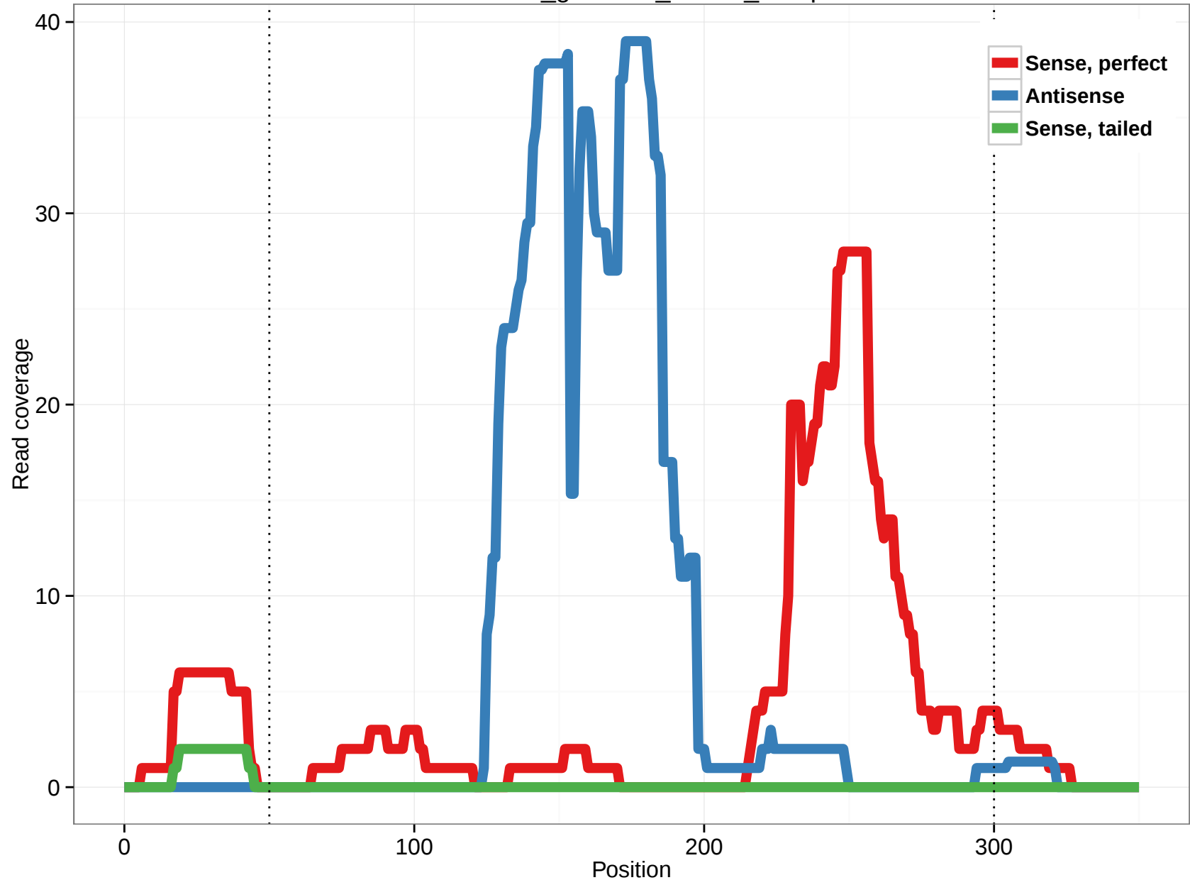
rheMac3_genscan_chr6.5_10.5p
