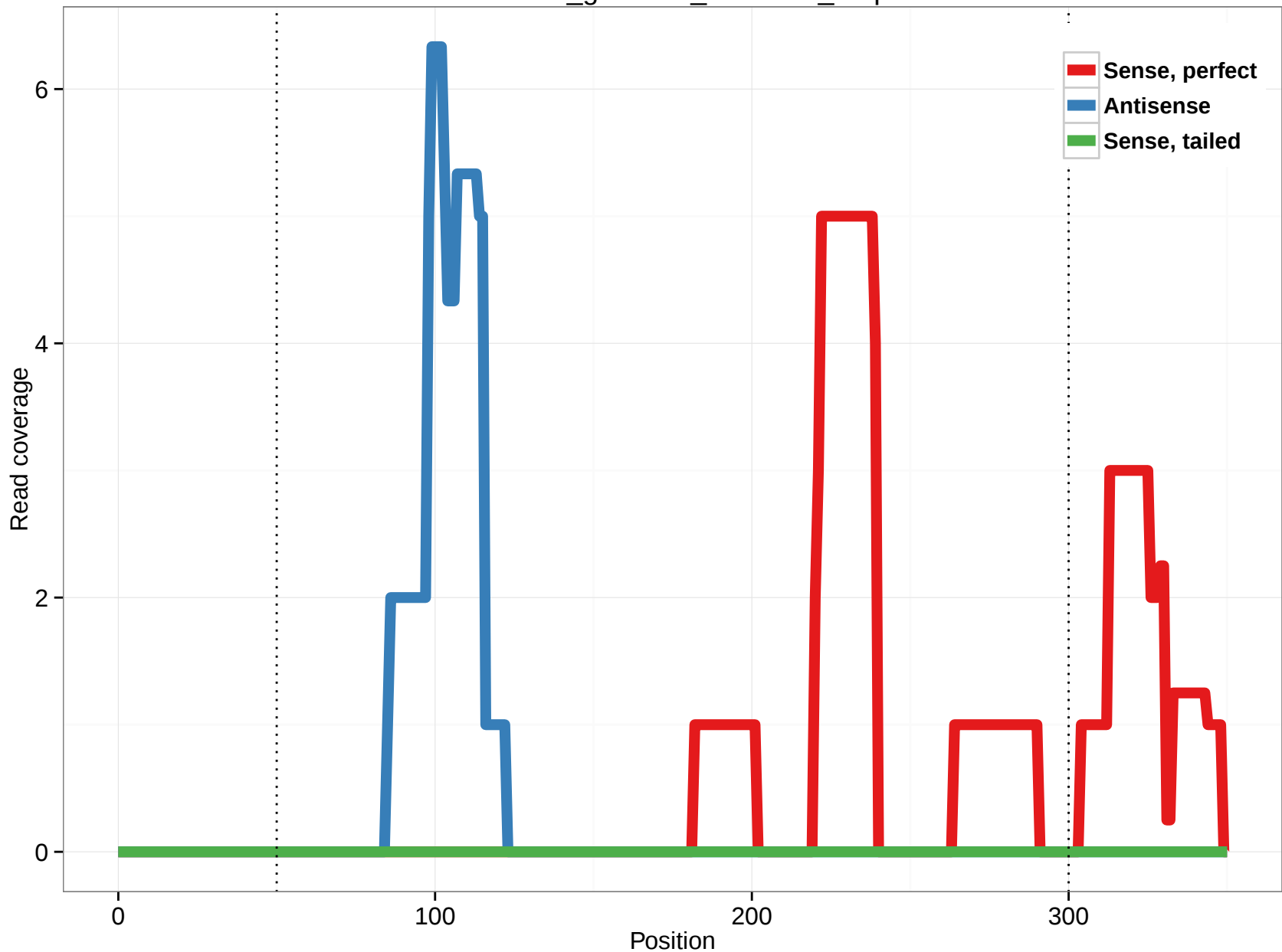
rheMac3_genscan_chr6.579_0.3p
