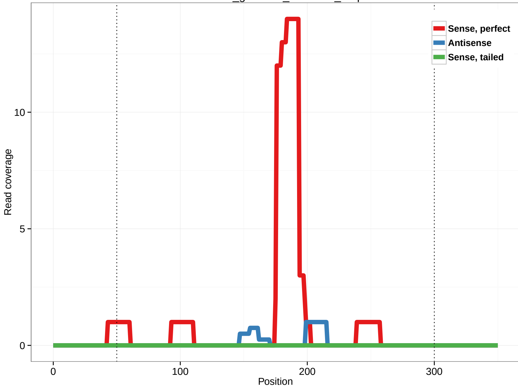
rheMac3_genscan_chr6.477_3.5p
