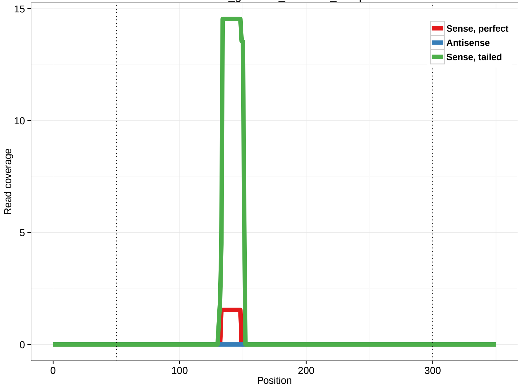
rheMac3_genscan_chr6.381_24.5p
