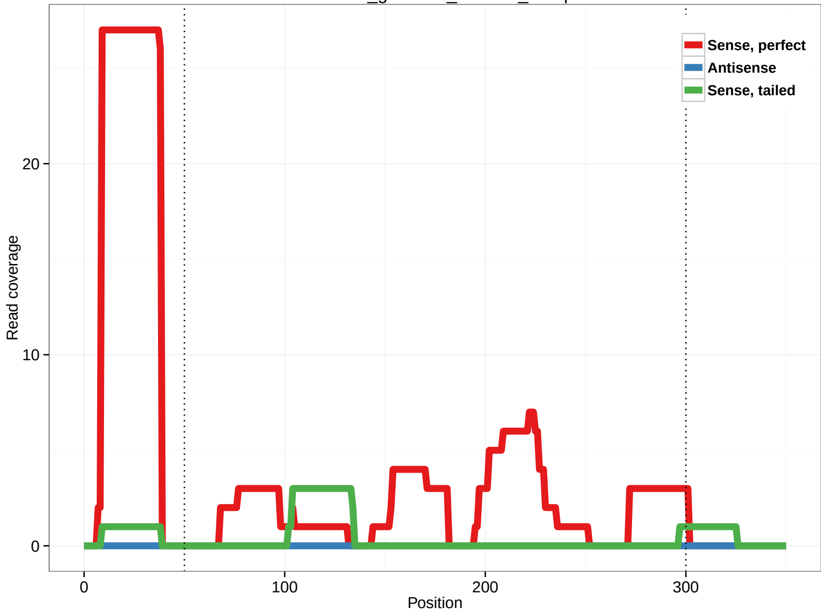
rheMac3_genscan_chr6.33_19.5p
