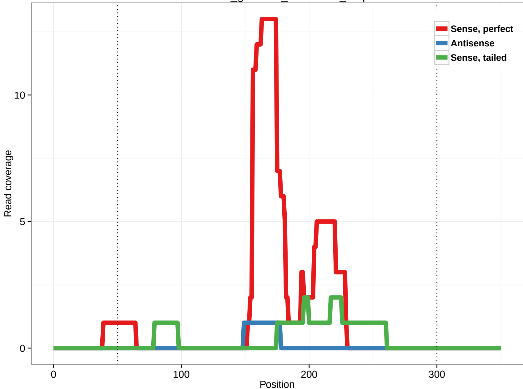
rheMac3_genscan_chr6.3131_6.5p
