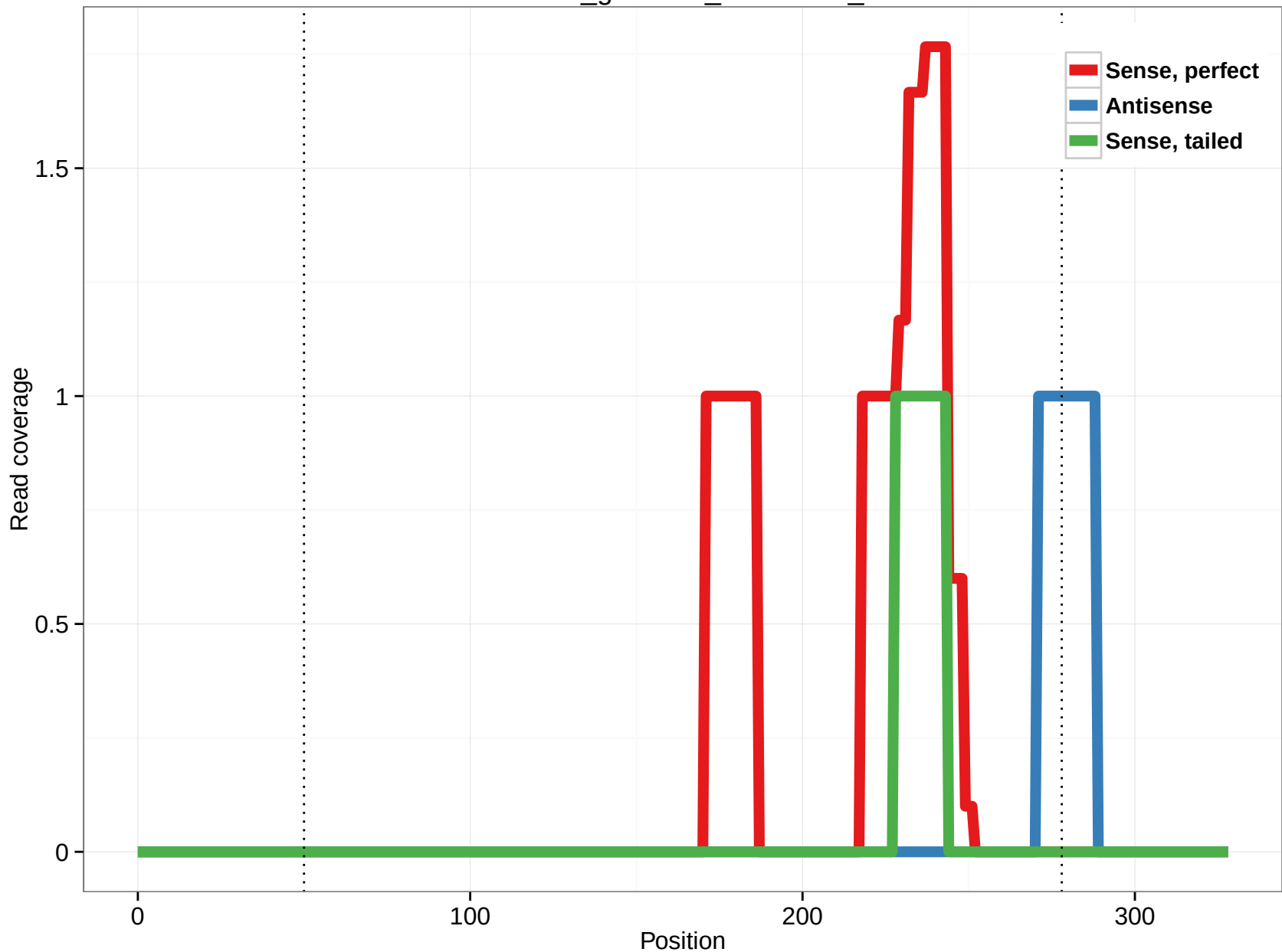
rheMac3_genscan_chr6.3095_13
