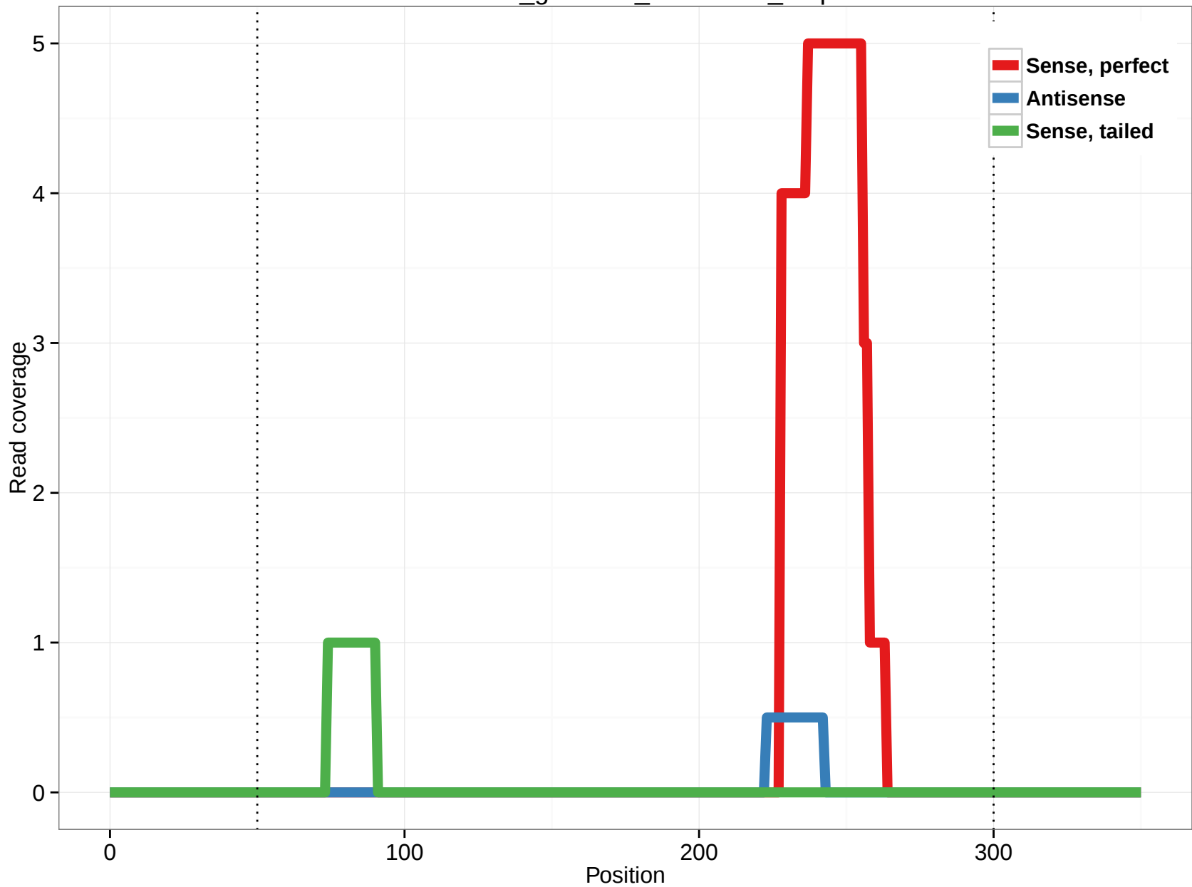
rheMac3_genscan_chr6.3092_5.3p
