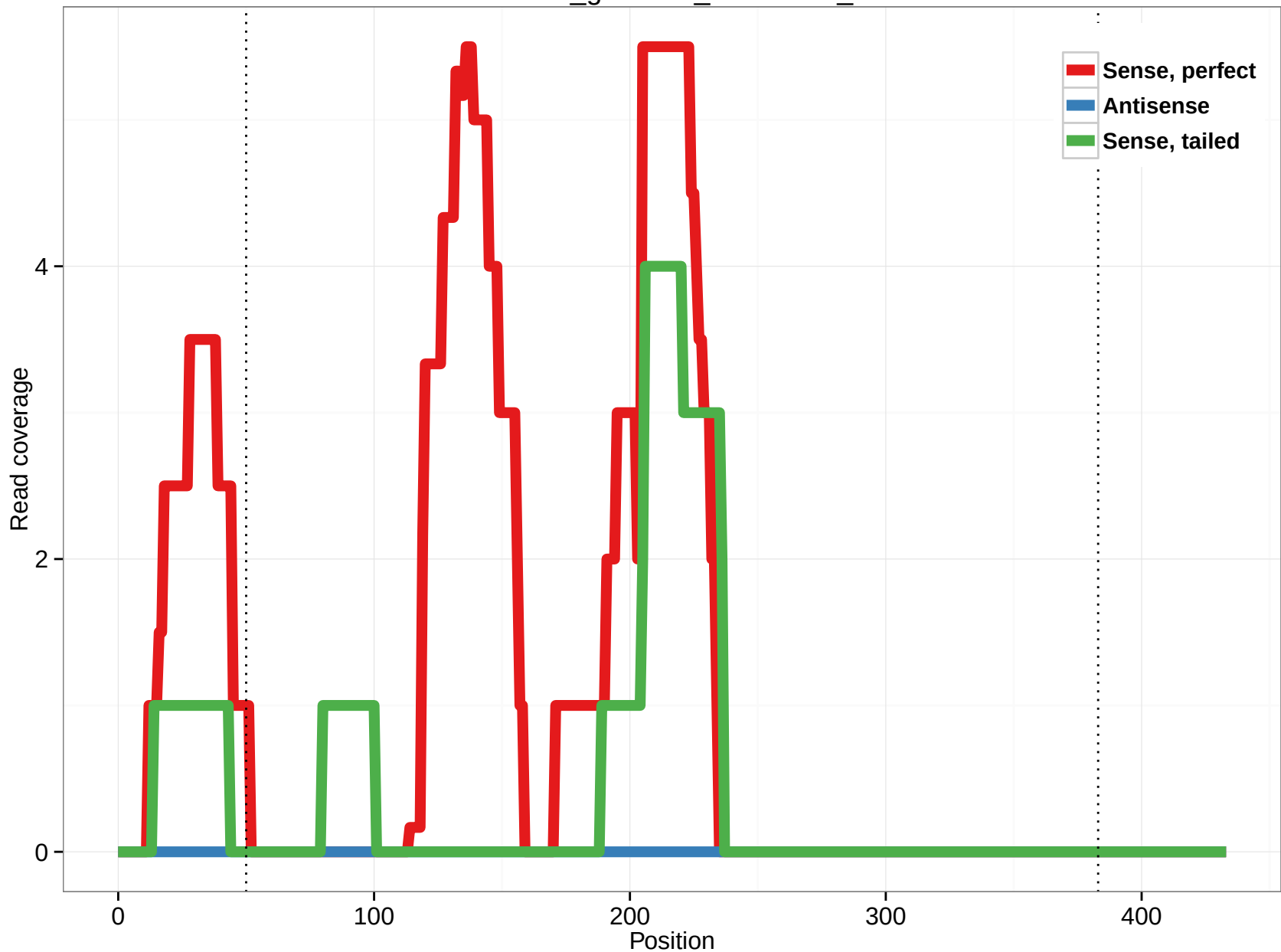
rheMac3_genscan_chr6.3092_21
