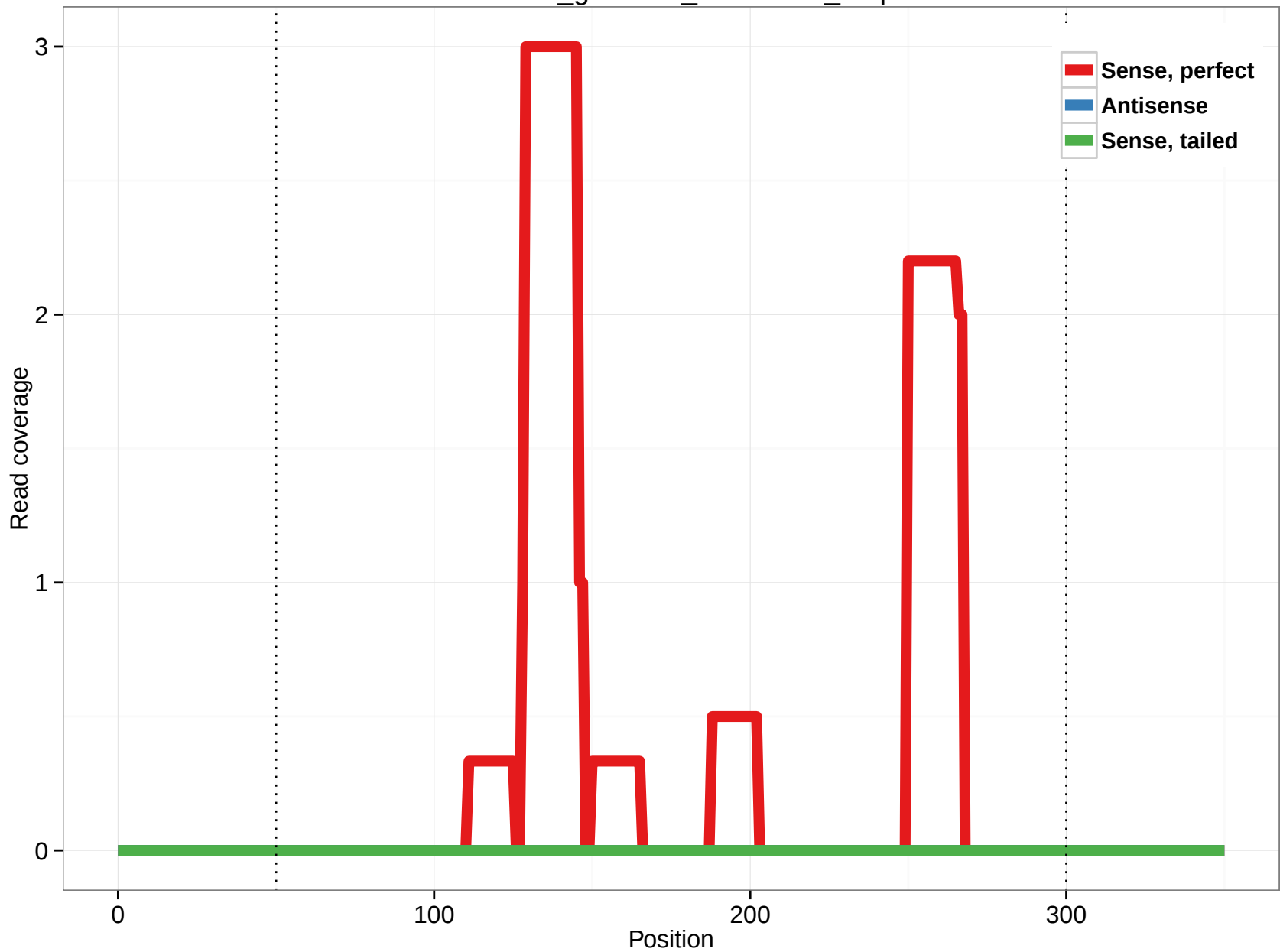
rheMac3_genscan_chr6.3092_1.5p
