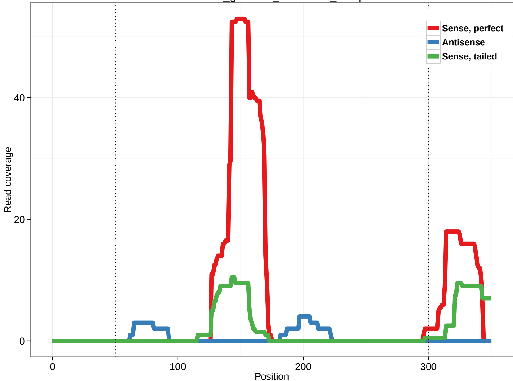
rheMac3_genscan_chr6.3091_24.3p
