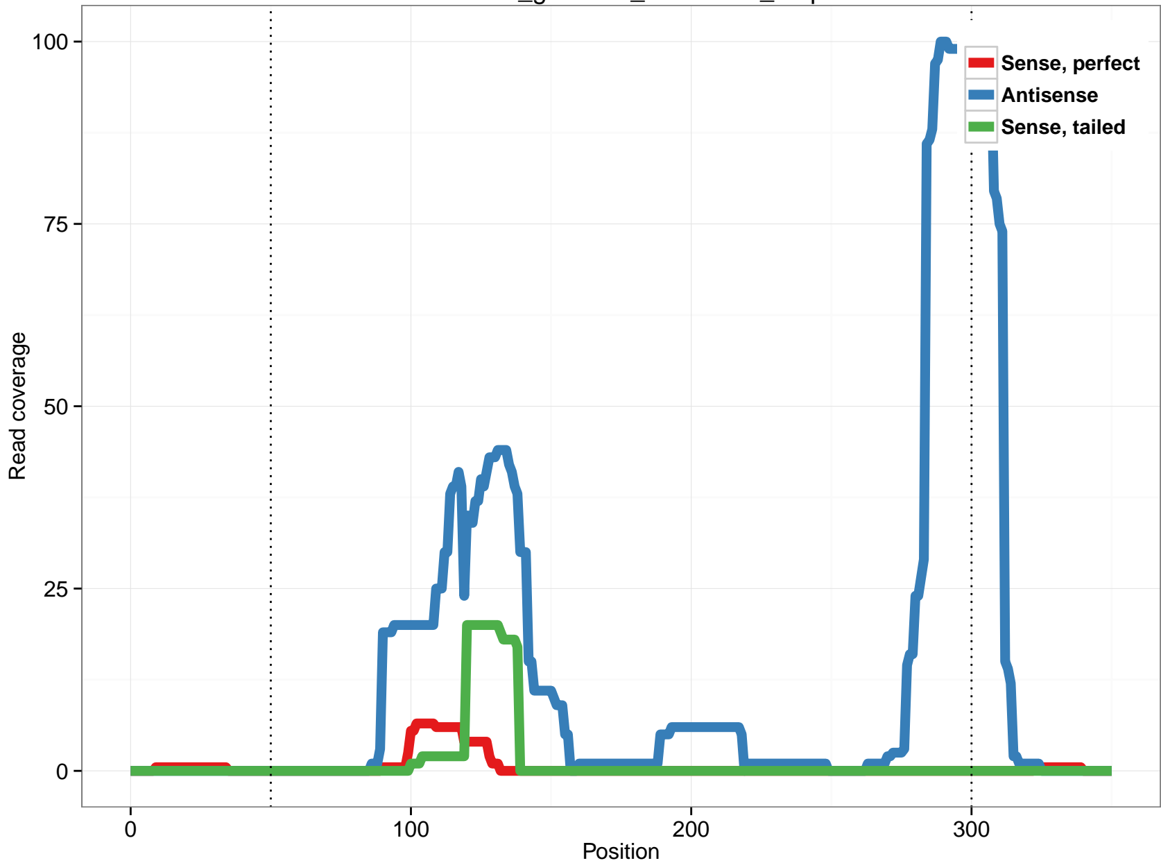
rheMac3_genscan_chr6.3041_7.5p
