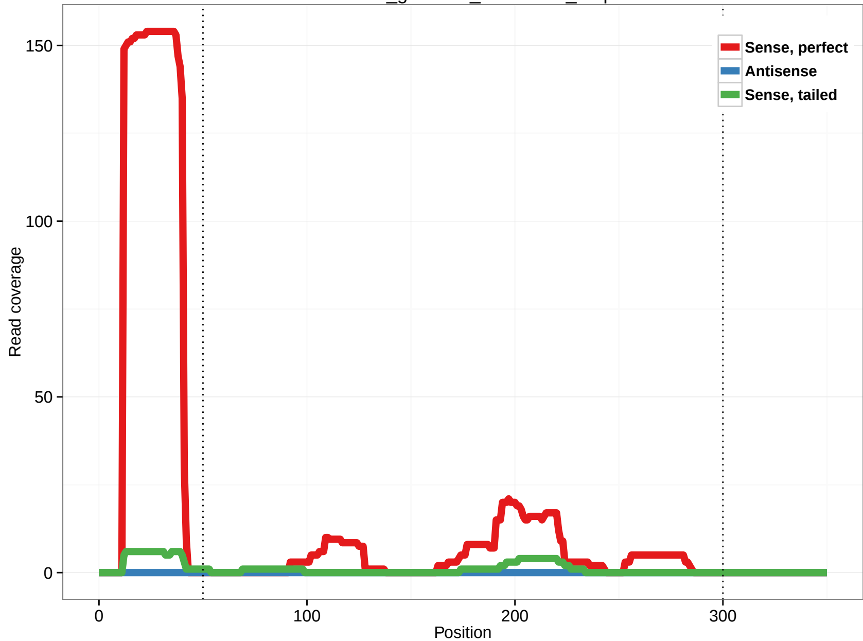
rheMac3_genscan_chr6.3040_7.3p
