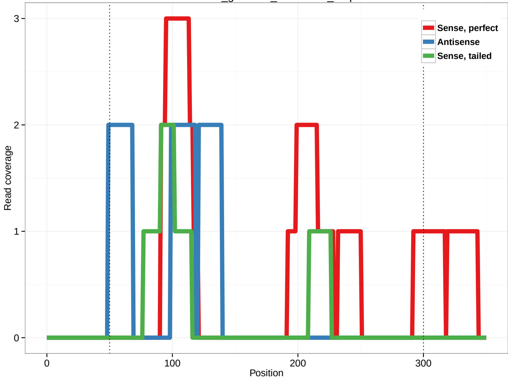
rheMac3_genscan_chr6.3008_9.3p
