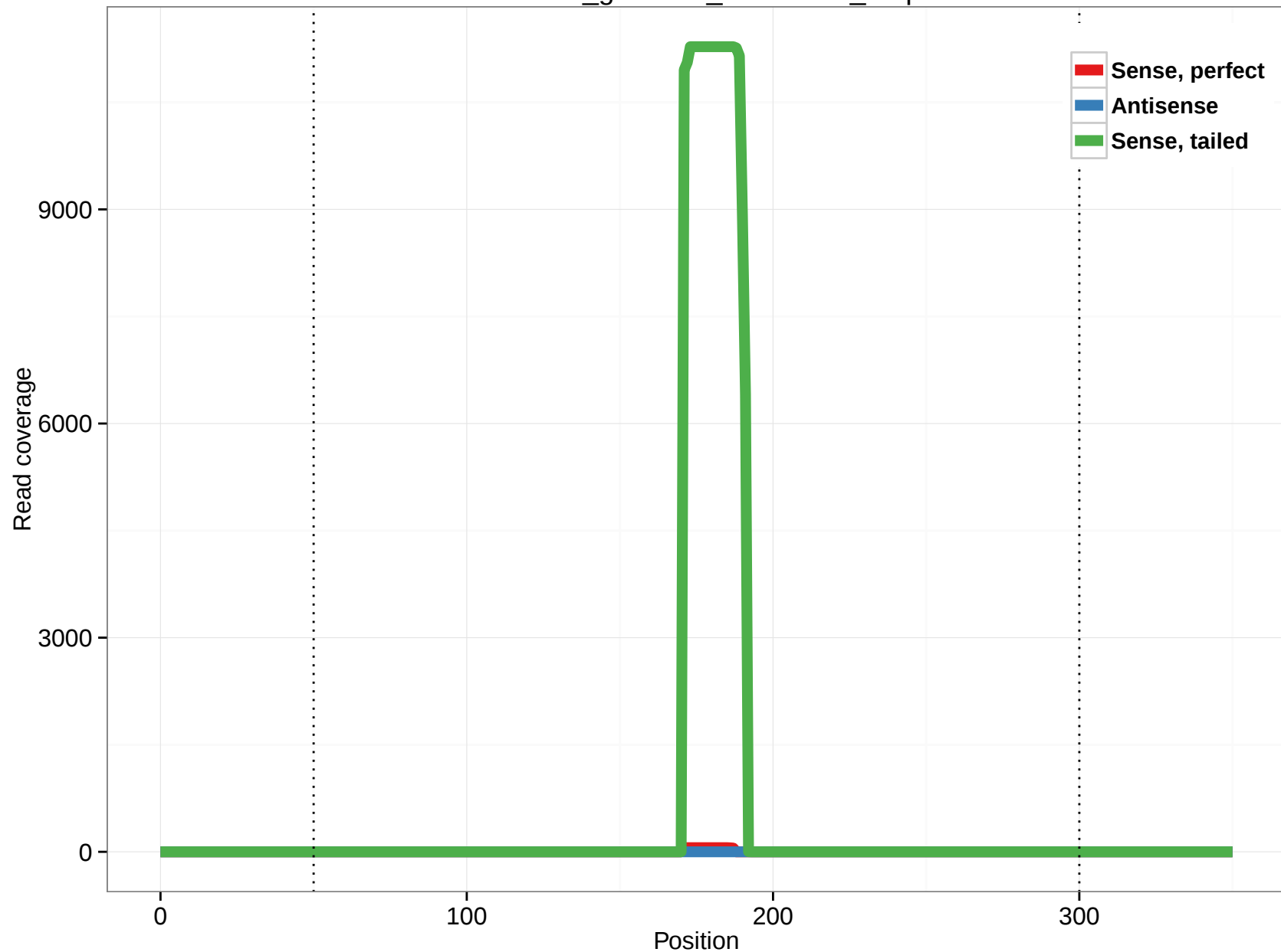
rheMac3_genscan_chr6.2970_4.3p
